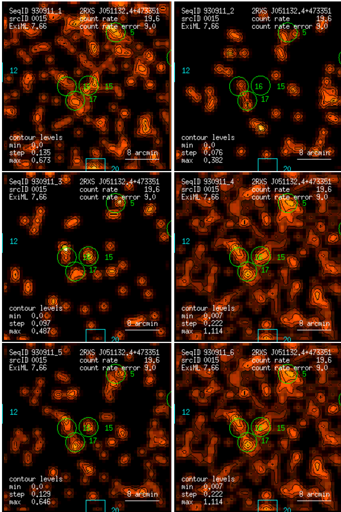
Figure 15: RASS 930911: detection 0015: band rate images, Gaussian filter: (1) PSPC channels 11 – 41, (2) 52 – 90, (3) 91 – 201, (4) 11 – 235, (5) 52 – 201, (6) 11 – 201. Broad band rates in counts/ks. Band rate contour levels in counts/ks/arcmin 2 .
