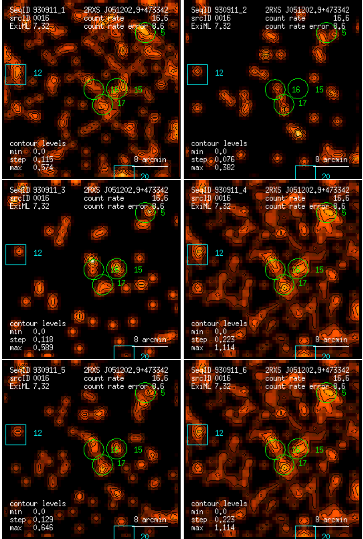
Figure 16: RASS 930911: detection 0016: band rate images, Gaussian filter: (1) PSPC channels 11 – 41, (2) 52 – 90, (3) 91 – 201, (4) 11 – 235, (5) 52 – 201, (6) 11 – 201. Broad band rates in counts/ks. Band rate contour levels in counts/ks/arcmin 2 .
