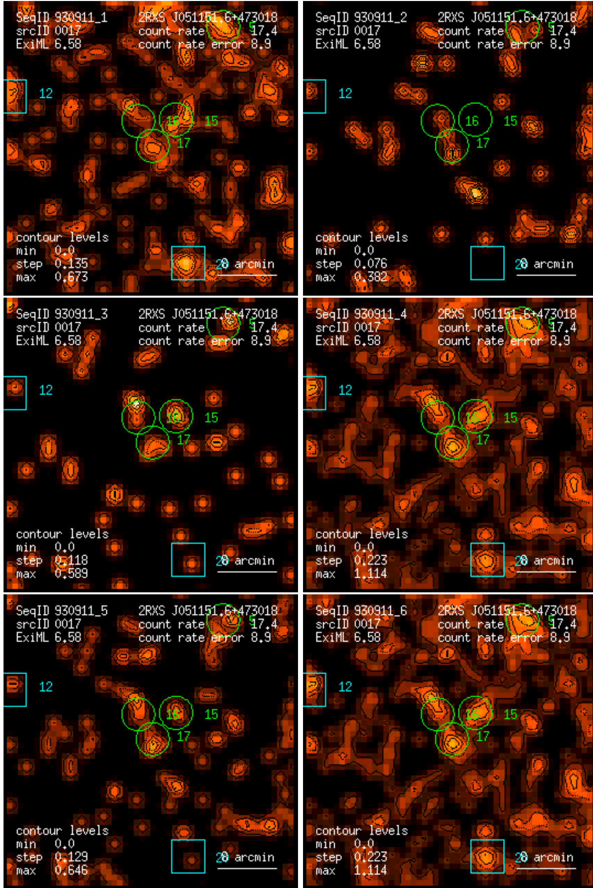
Figure 17: RASS 930911: detection 0017: band rate images, Gaussian filter: (1) PSPC channels 11 – 41, (2) 52 – 90, (3) 91 – 201, (4) 11 – 235, (5) 52 – 201, (6) 11 – 201. Broad band rates in counts/ks. Band rate contour levels in counts/ks/arcmin 2 .
