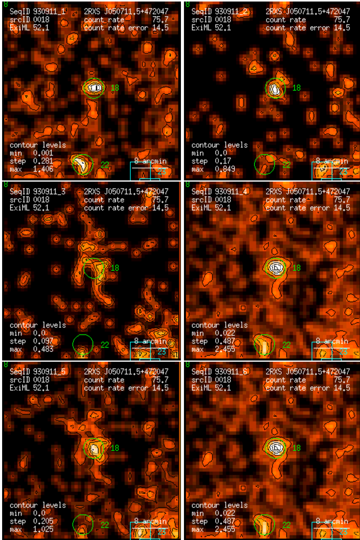
Figure 18: RASS 930911: detection 0018: band rate images, Gaussian filter: (1) PSPC channels 11 – 41, (2) 52 – 90, (3) 91 – 201, (4) 11 – 235, (5) 52 – 201, (6) 11 – 201. Broad band rates in counts/ks. Band rate contour levels in counts/ks/arcmin 2 .
