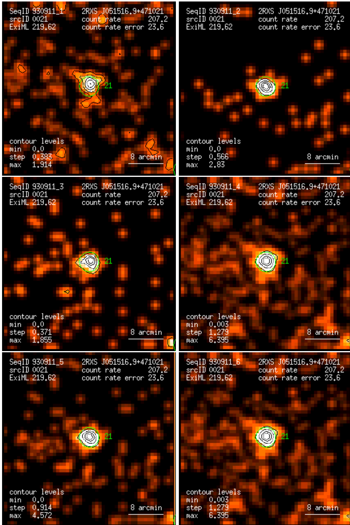
Figure 21: RASS 930911: detection 0021: band rate images, Gaussian filter: (1) PSPC channels 11 – 41, (2) 52 – 90, (3) 91 – 201, (4) 11 – 235, (5) 52 – 201, (6) 11 – 201. Broad band rates in counts/ks. Band rate contour levels in counts/ks/arcmin 2 .
