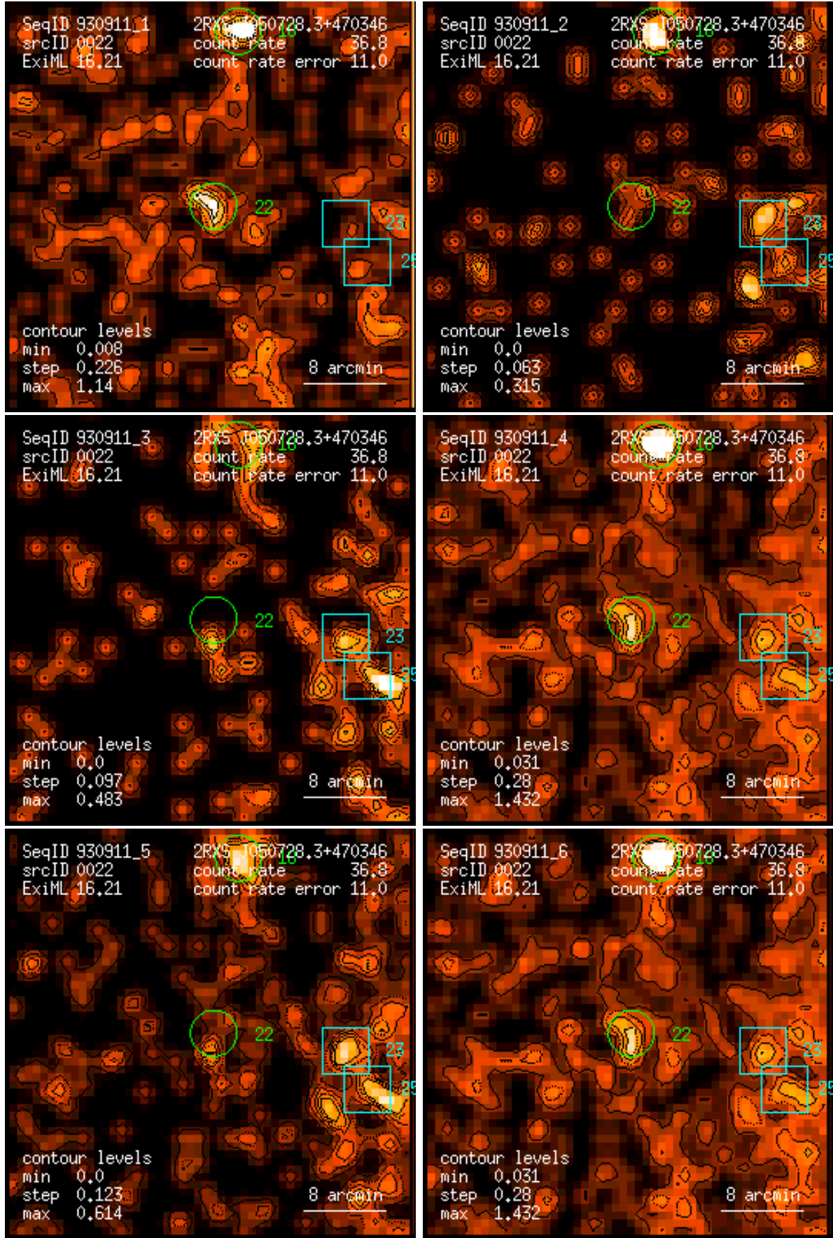
Figure 22: RASS 930911: detection 0022: band rate images, Gaussian filter: (1) PSPC channels 11 – 41, (2) 52 – 90, (3) 91 – 201, (4) 11 – 235, (5) 52 – 201, (6) 11 – 201. Broad band rates in counts/ks. Band rate contour levels in counts/ks/arcmin 2 .
