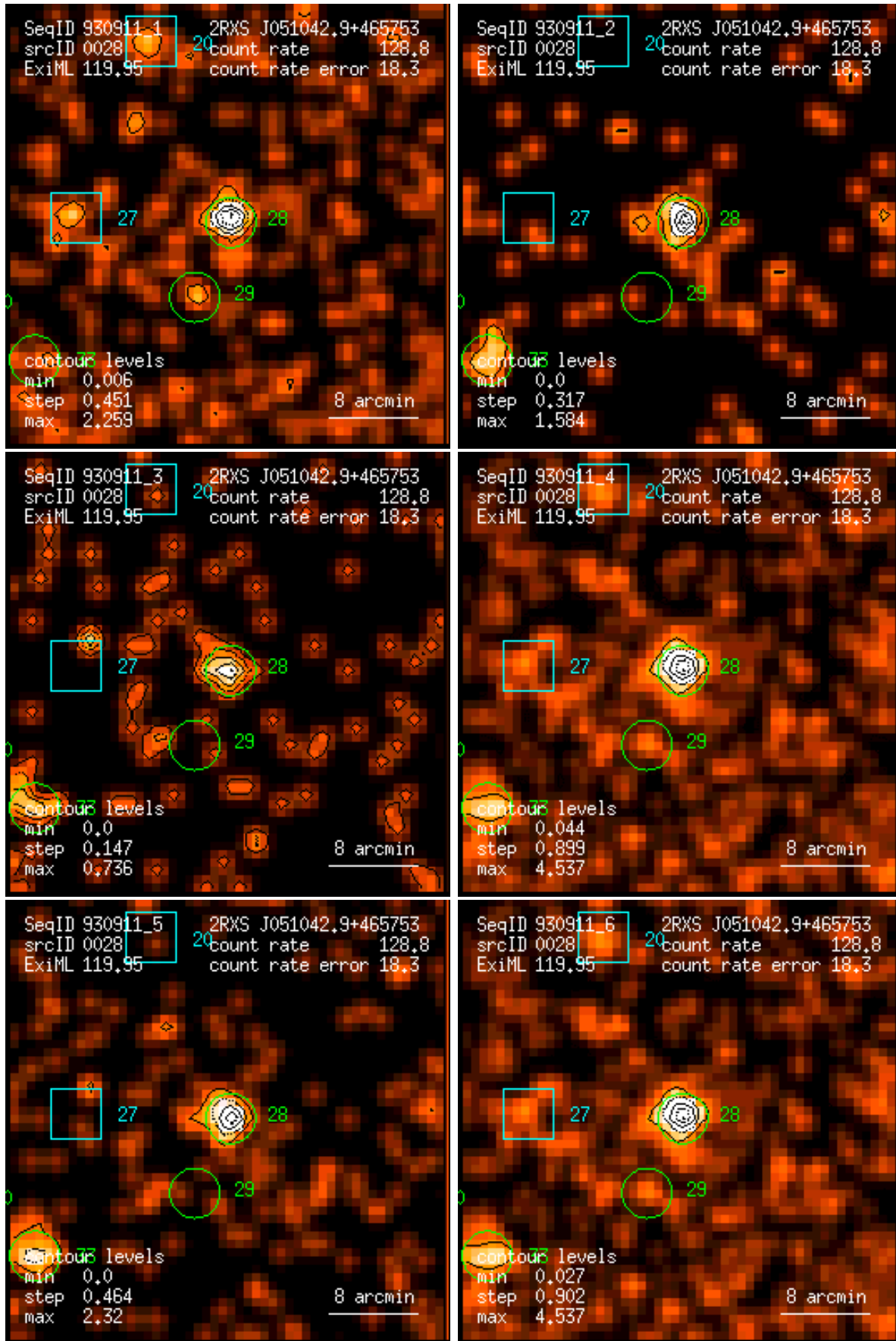
Figure 28: RASS 930911: detection 0028: band rate images, Gaussian filter: (1) PSPC channels 11 – 41, (2) 52 – 90, (3) 91 – 201, (4) 11 – 235, (5) 52 – 201, (6) 11 – 201. Broad band rates in counts/ks. Band rate contour levels in counts/ks/arcmin 2 .
