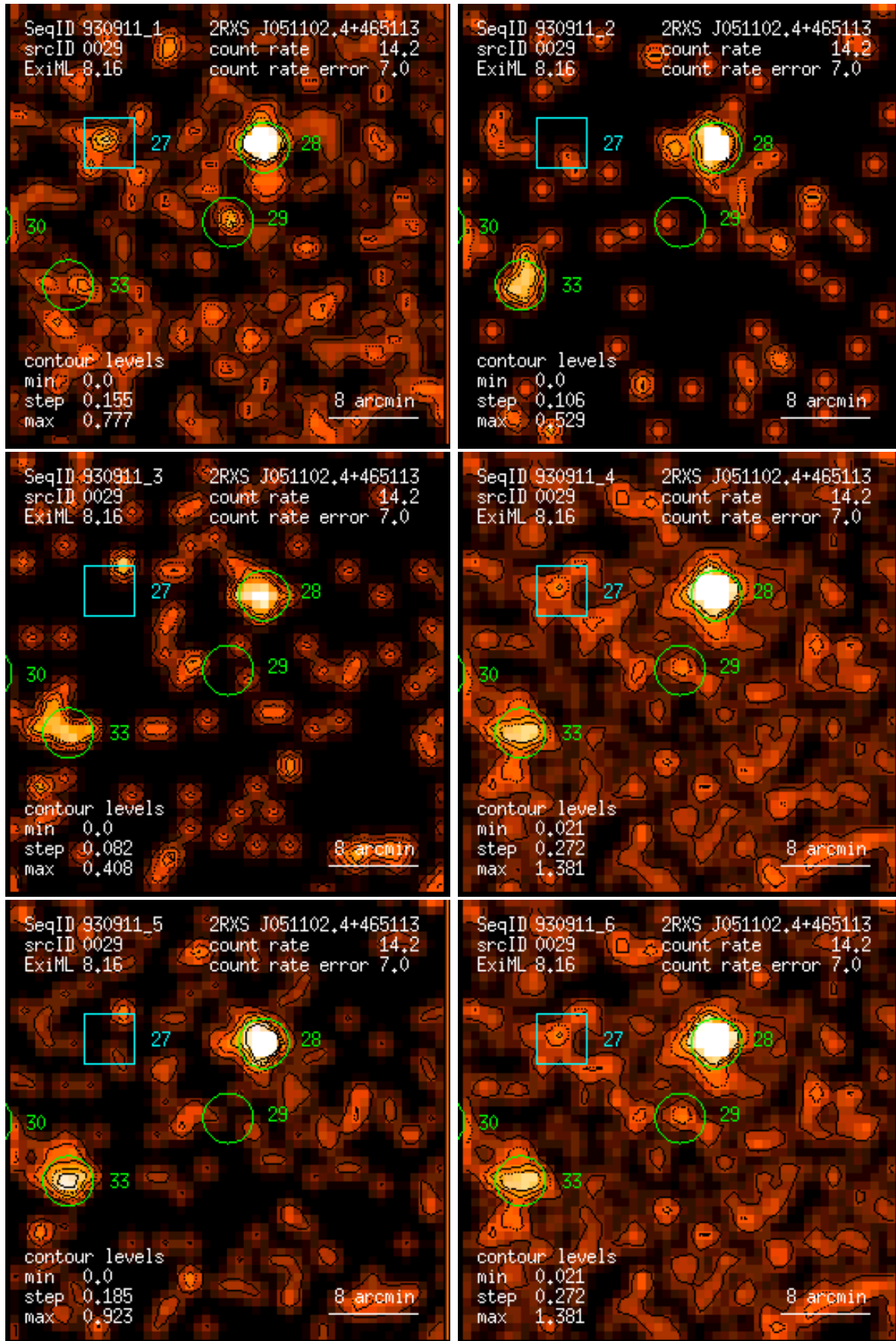
Figure 29: RASS 930911: detection 0029: band rate images, Gaussian filter: (1) PSPC channels 11 – 41, (2) 52 – 90, (3) 91 – 201, (4) 11 – 235, (5) 52 – 201, (6) 11 – 201. Broad band rates in counts/ks. Band rate contour levels in counts/ks/arcmin 2 .
