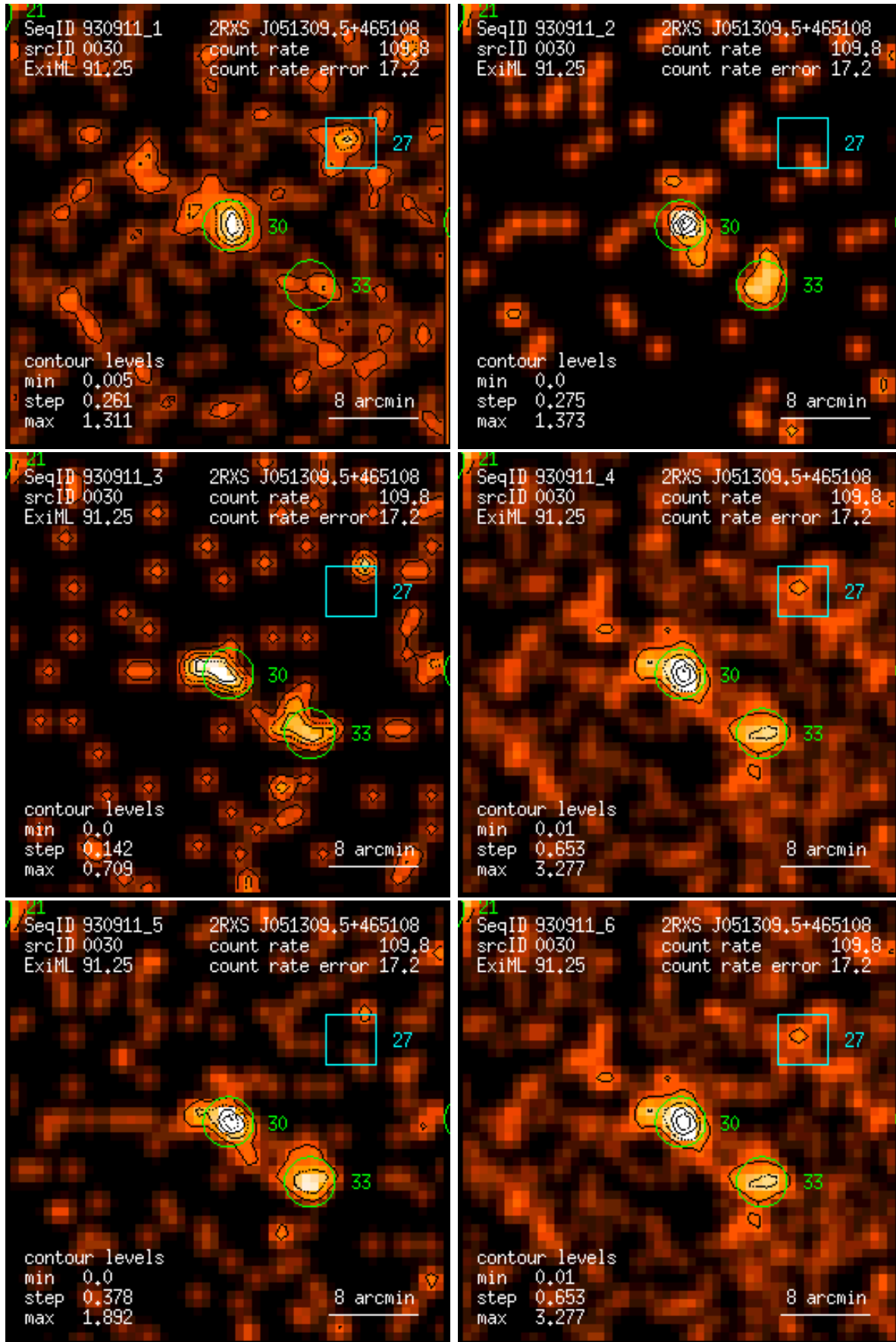
Figure 30: RASS 930911: detection 0030: band rate images, Gaussian filter: (1) PSPC channels 11 – 41, (2) 52 – 90, (3) 91 – 201, (4) 11 – 235, (5) 52 – 201, (6) 11 – 201. Broad band rates in counts/ks. Band rate contour levels in counts/ks/arcmin 2 .
