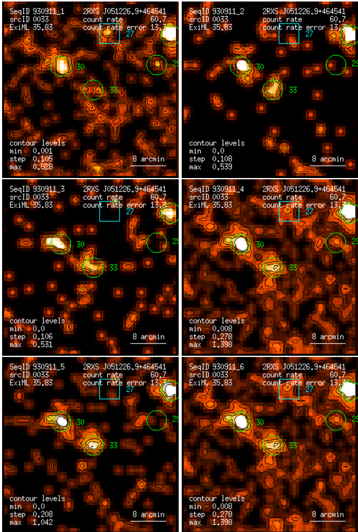
Figure 33: RASS 930911: detection 0033: band rate images, Gaussian filter: (1) PSPC channels 11 – 41, (2) 52 – 90, (3) 91 – 201, (4) 11 – 235, (5) 52 – 201, (6) 11 – 201. Broad band rates in counts/ks. Band rate contour levels in counts/ks/arcmin 2 .
