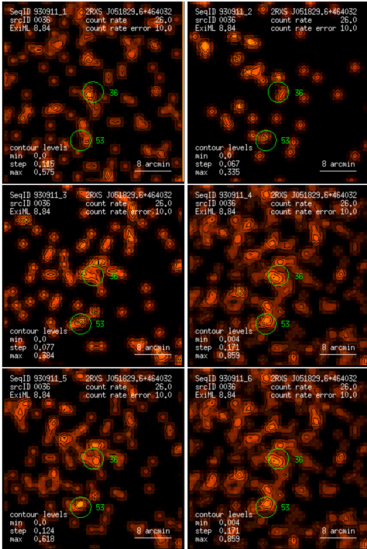
Figure 36: RASS 930911: detection 0036: band rate images, Gaussian filter: (1) PSPC channels 11 – 41, (2) 52 – 90, (3) 91 – 201, (4) 11 – 235, (5) 52 – 201, (6) 11 – 201. Broad band rates in counts/ks. Band rate contour levels in counts/ks/arcmin 2 .
