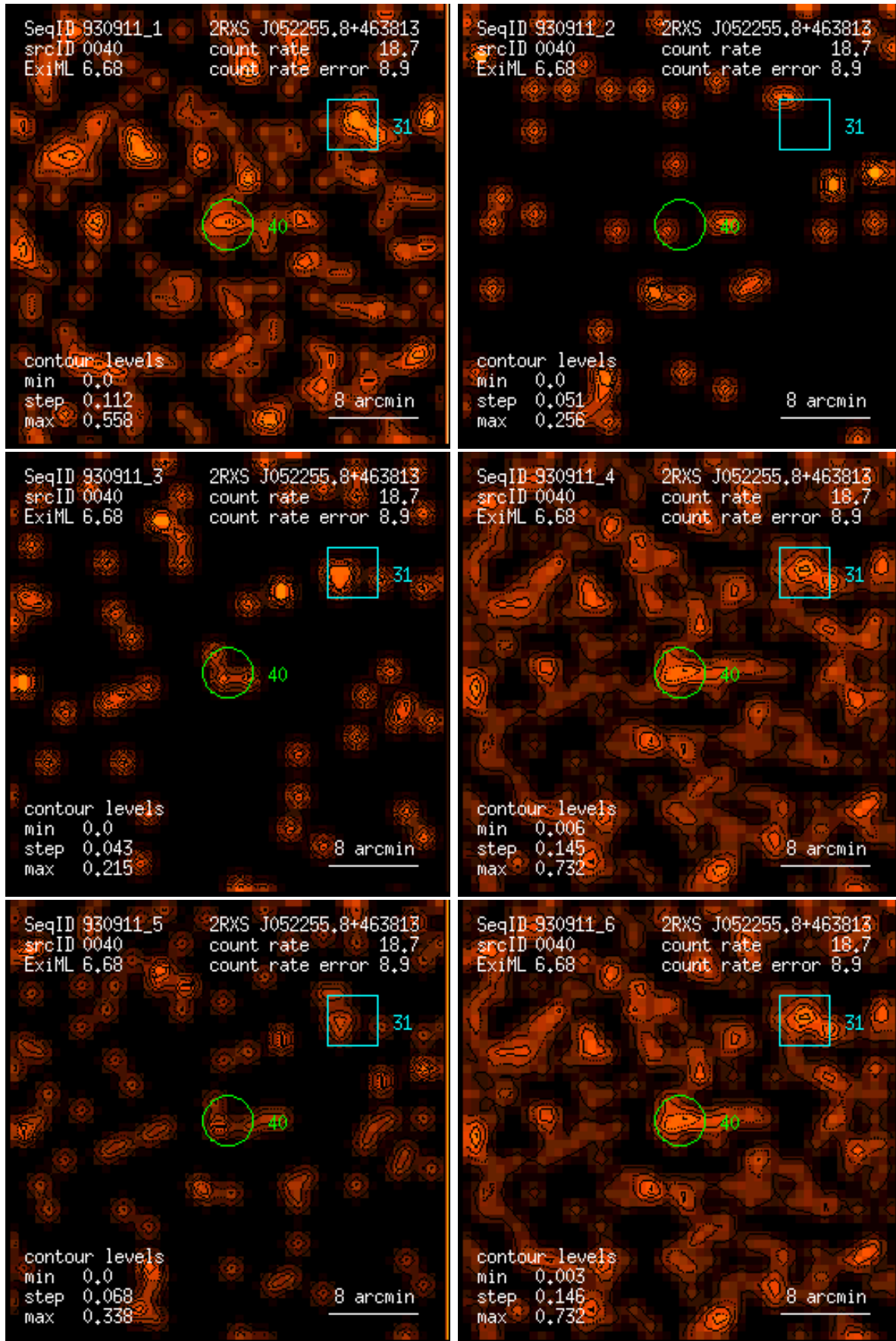
Figure 40: RASS 930911: detection 0040: band rate images, Gaussian filter: (1) PSPC channels 11 – 41, (2) 52 – 90, (3) 91 – 201, (4) 11 – 235, (5) 52 – 201, (6) 11 – 201. Broad band rates in counts/ks. Band rate contour levels in counts/ks/arcmin 2 .
