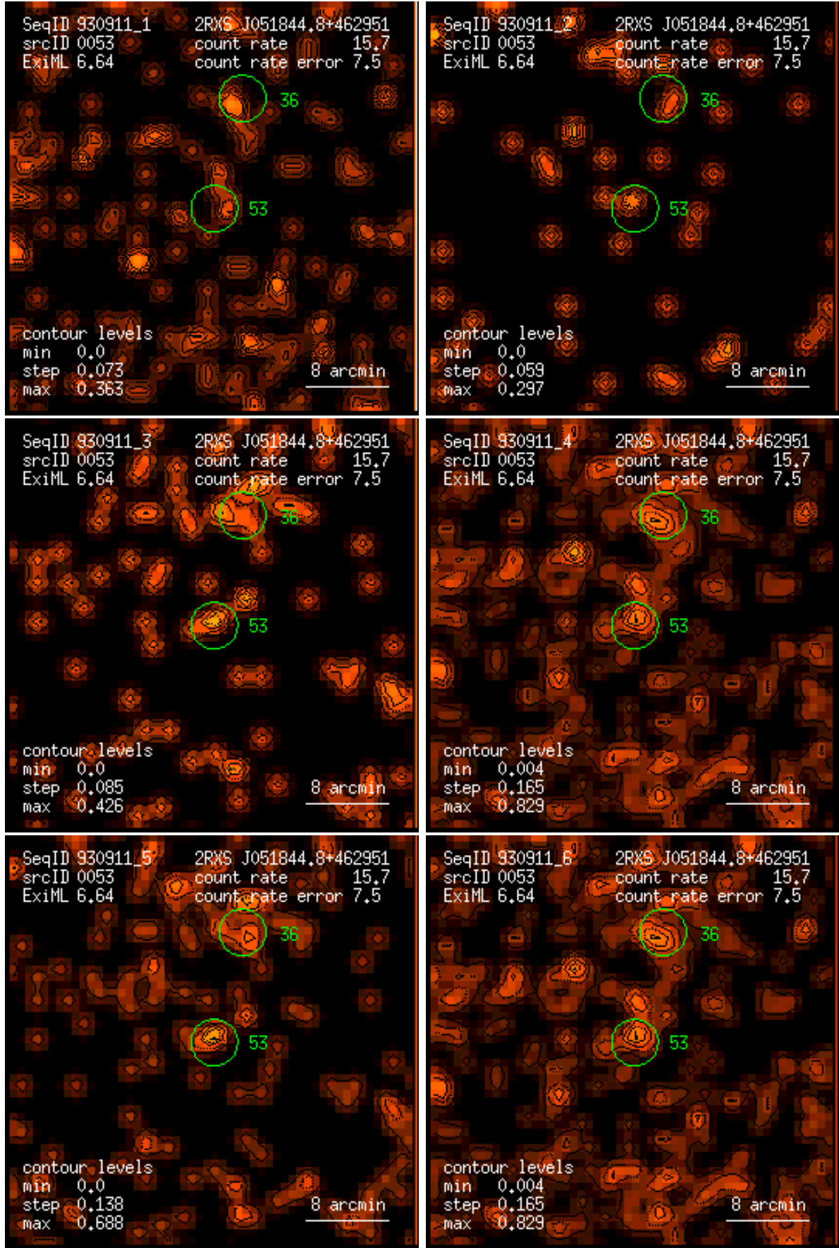
Figure 53: RASS 930911: detection 0053: band rate images, Gaussian filter: (1) PSPC channels 11 – 41, (2) 52 – 90, (3) 91 – 201, (4) 11 – 235, (5) 52 – 201, (6) 11 – 201. Broad band rates in counts/ks. Band rate contour levels in counts/ks/arcmin 2 .
