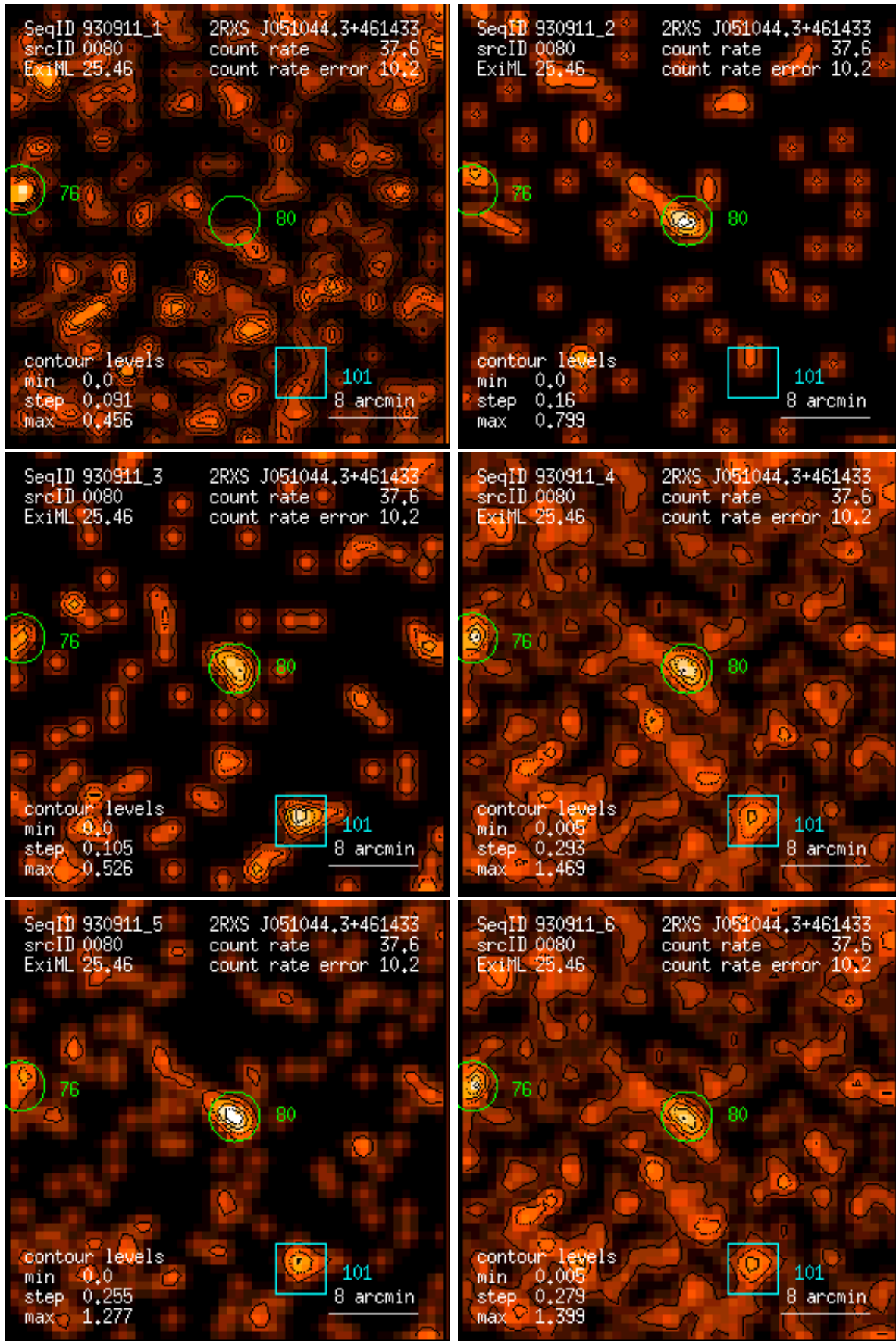
Figure 80: RASS 930911: detection 0080: band rate images, Gaussian filter: (1) PSPC channels 11 – 41, (2) 52 – 90, (3) 91 – 201, (4) 11 – 235, (5) 52 – 201, (6) 11 – 201. Broad band rates in counts/ks. Band rate contour levels in counts/ks/arcmin 2 .
