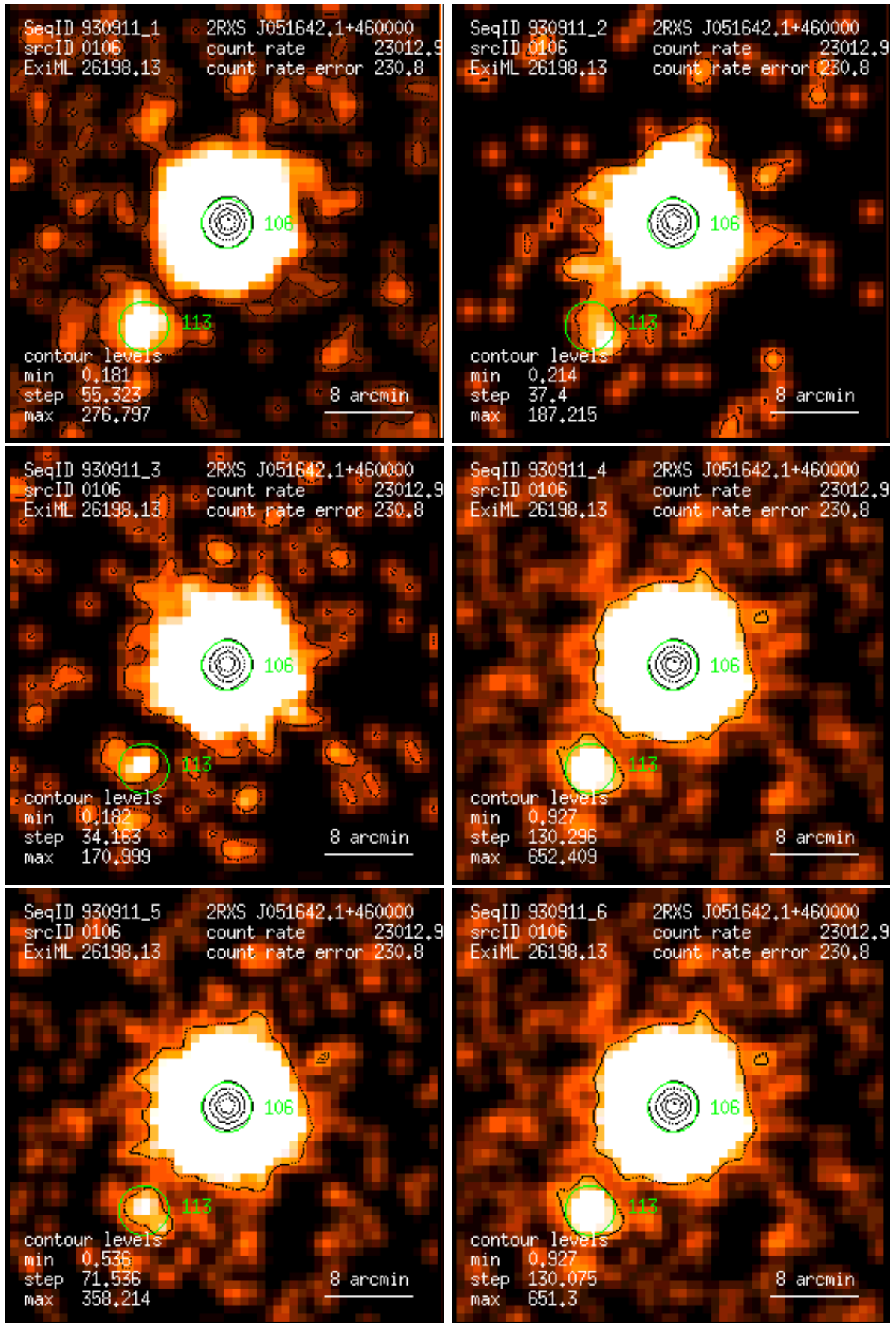
Figure 106: RASS 930911: detection 0106: band rate images, Gaussian filter: (1) PSPC channels 11 – 41, (2) 52 – 90, (3) 91 – 201, (4) 11 – 235, (5) 52 – 201, (6) 11 – 201. Broad band rates in counts/ks. Band rate contour levels in counts/ks/arcmin 2 .
