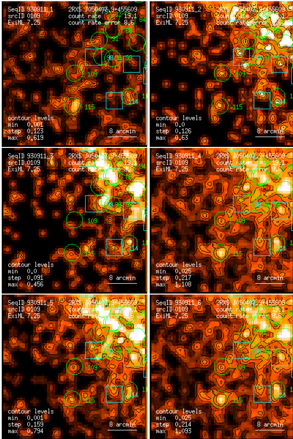
Figure 109: RASS 930911: detection 0109: band rate images, Gaussian filter: (1) PSPC channels 11 – 41, (2) 52 – 90, (3) 91 – 201, (4) 11 – 235, (5) 52 – 201, (6) 11 – 201. Broad band rates in counts/ks. Band rate contour levels in counts/ks/arcmin 2 .
