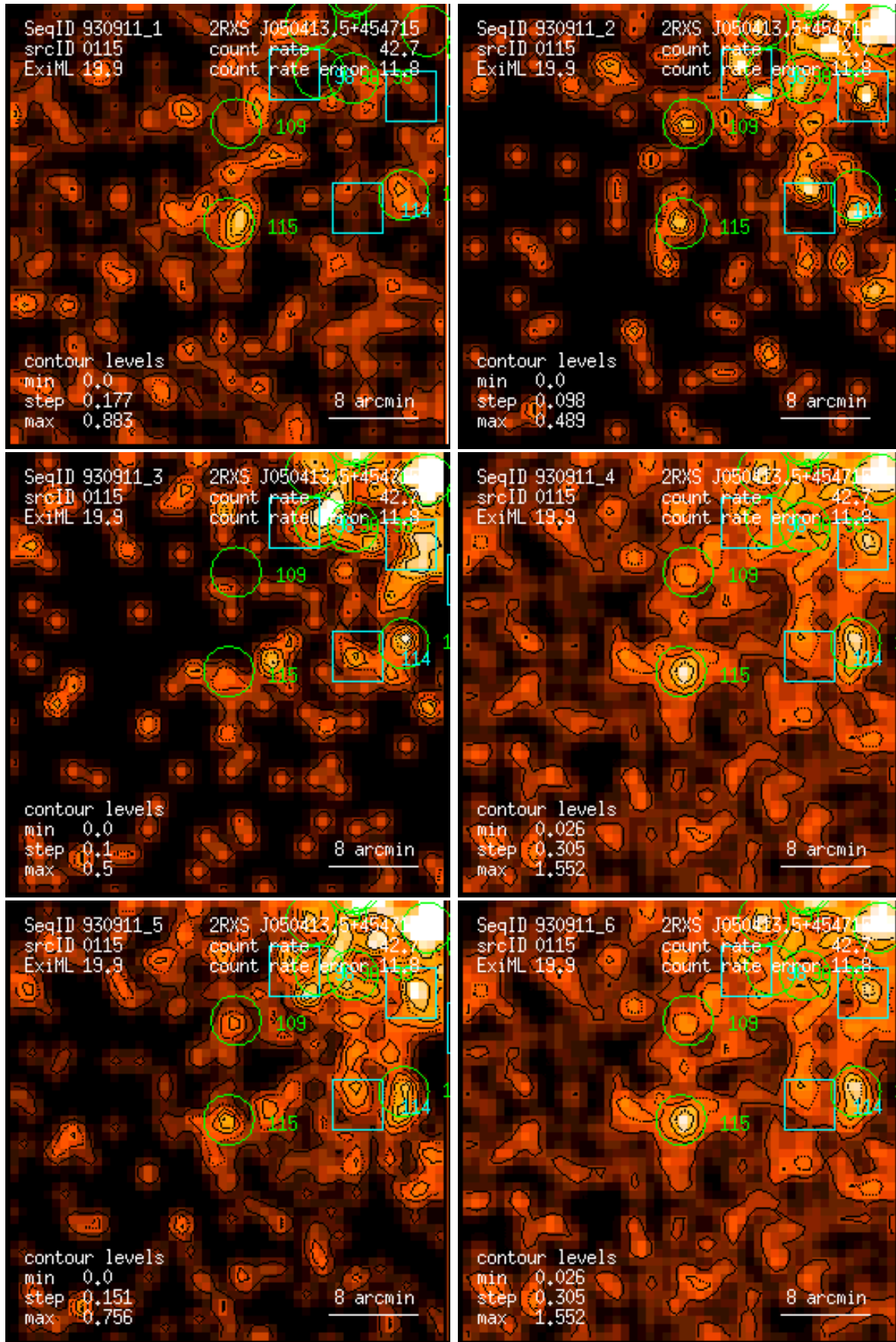
Figure 115: RASS 930911: detection 0115: band rate images, Gaussian filter: (1) PSPC channels 11 – 41, (2) 52 – 90, (3) 91 – 201, (4) 11 – 235, (5) 52 – 201, (6) 11 – 201. Broad band rates in counts/ks. Band rate contour levels in counts/ks/arcmin 2 .
