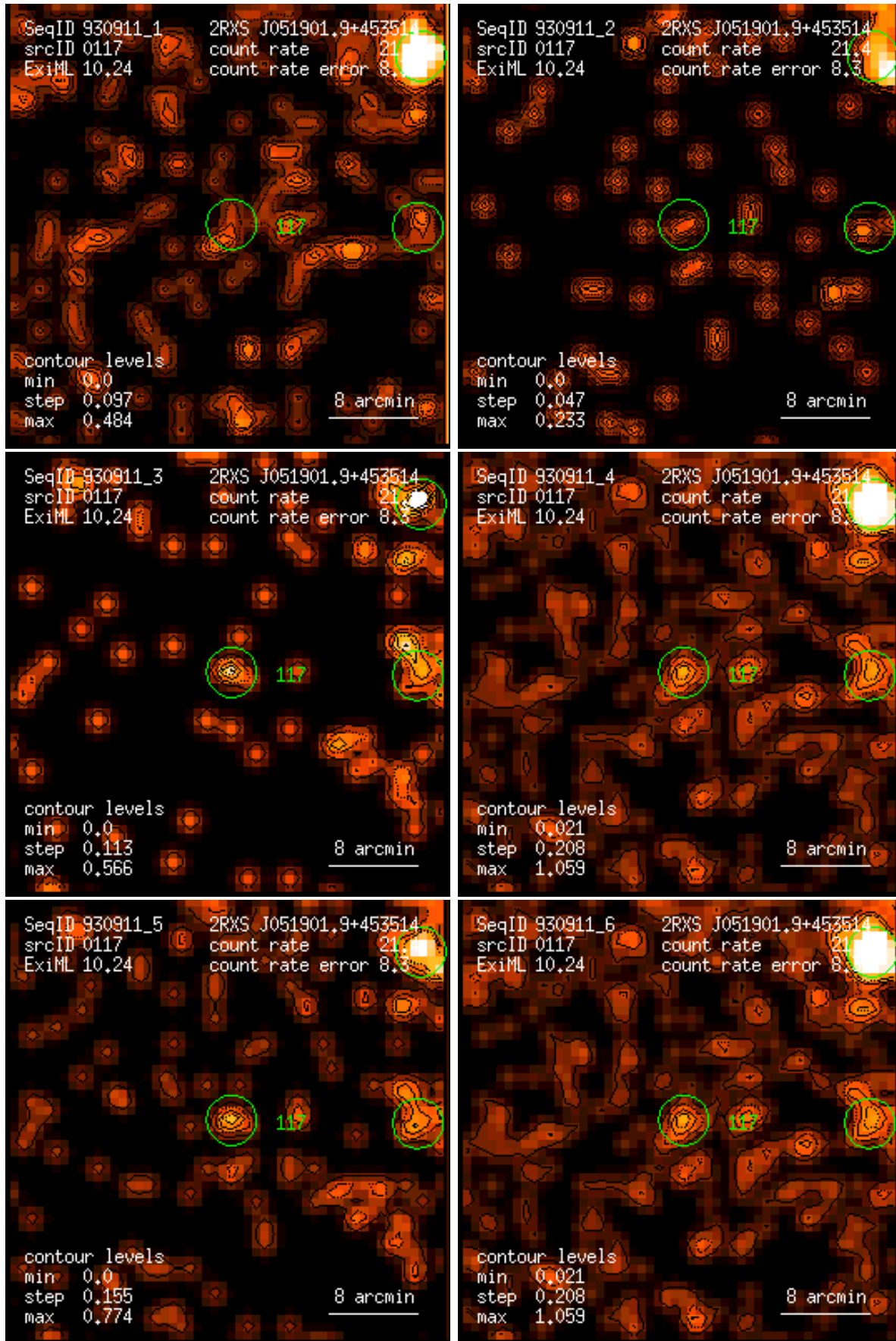
Figure 117: RASS 930911: detection 0117: band rate images, Gaussian filter: (1) PSPC channels 11 – 41, (2) 52 – 90, (3) 91 – 201, (4) 11 – 235, (5) 52 – 201, (6) 11 – 201. Broad band rates in counts/ks. Band rate contour levels in counts/ks/arcmin 2 .
