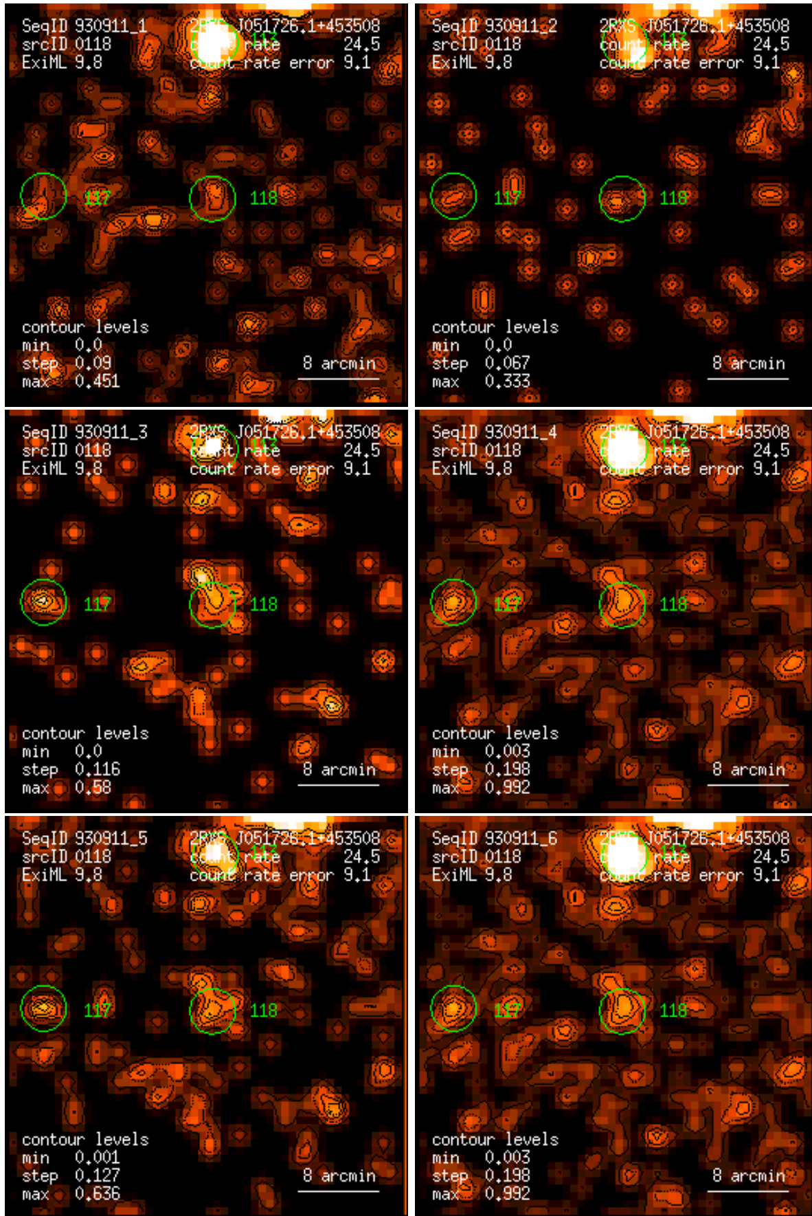
Figure 118: RASS 930911: detection 0118: band rate images, Gaussian filter: (1) PSPC channels 11 – 41, (2) 52 – 90, (3) 91 – 201, (4) 11 – 235, (5) 52 – 201, (6) 11 – 201. Broad band rates in counts/ks. Band rate contour levels in counts/ks/arcmin 2 .
