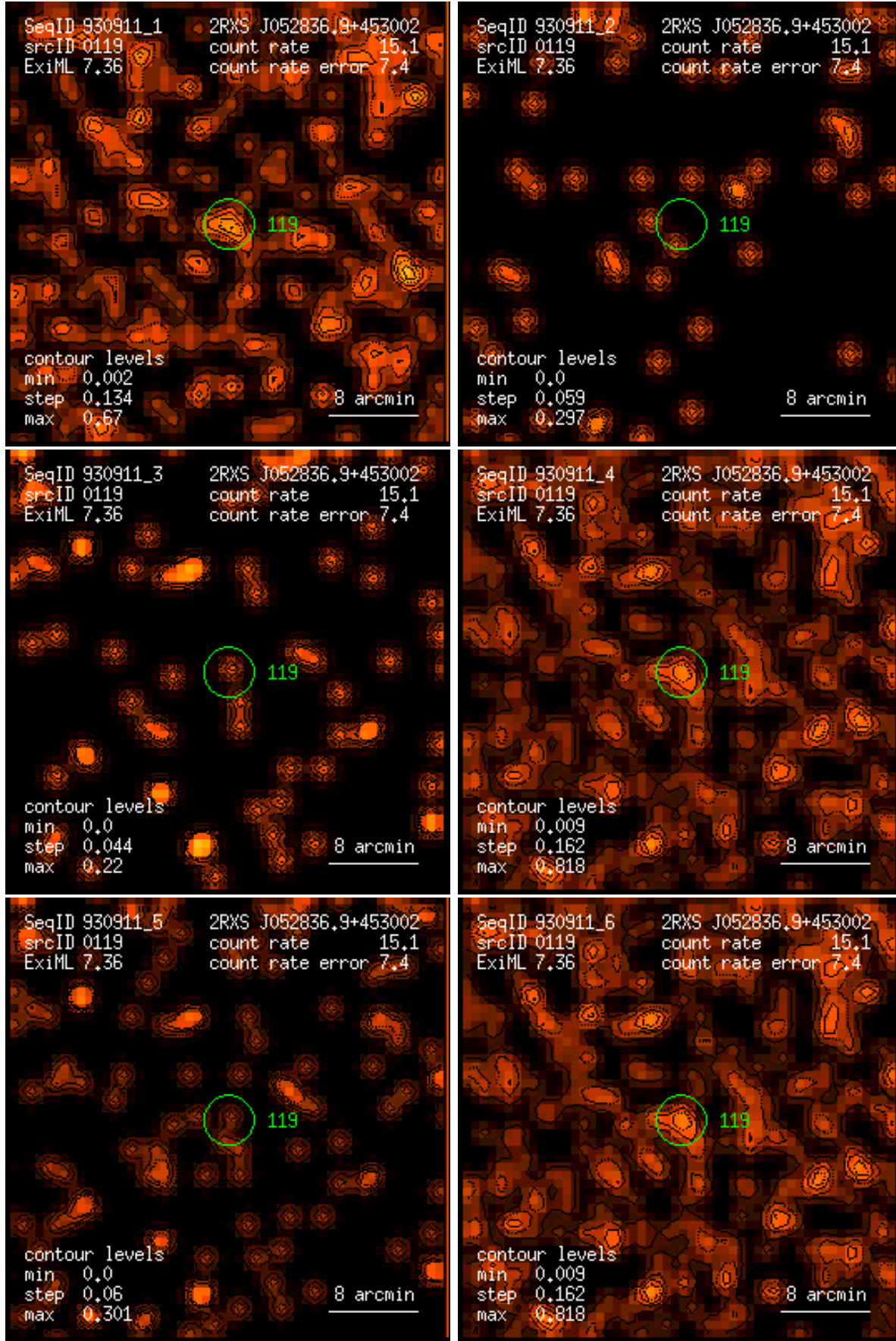
Figure 119: RASS 930911: detection 0119: band rate images, Gaussian filter: (1) PSPC channels 11 – 41, (2) 52 – 90, (3) 91 – 201, (4) 11 – 235, (5) 52 – 201, (6) 11 – 201. Broad band rates in counts/ks. Band rate contour levels in counts/ks/arcmin 2 .
