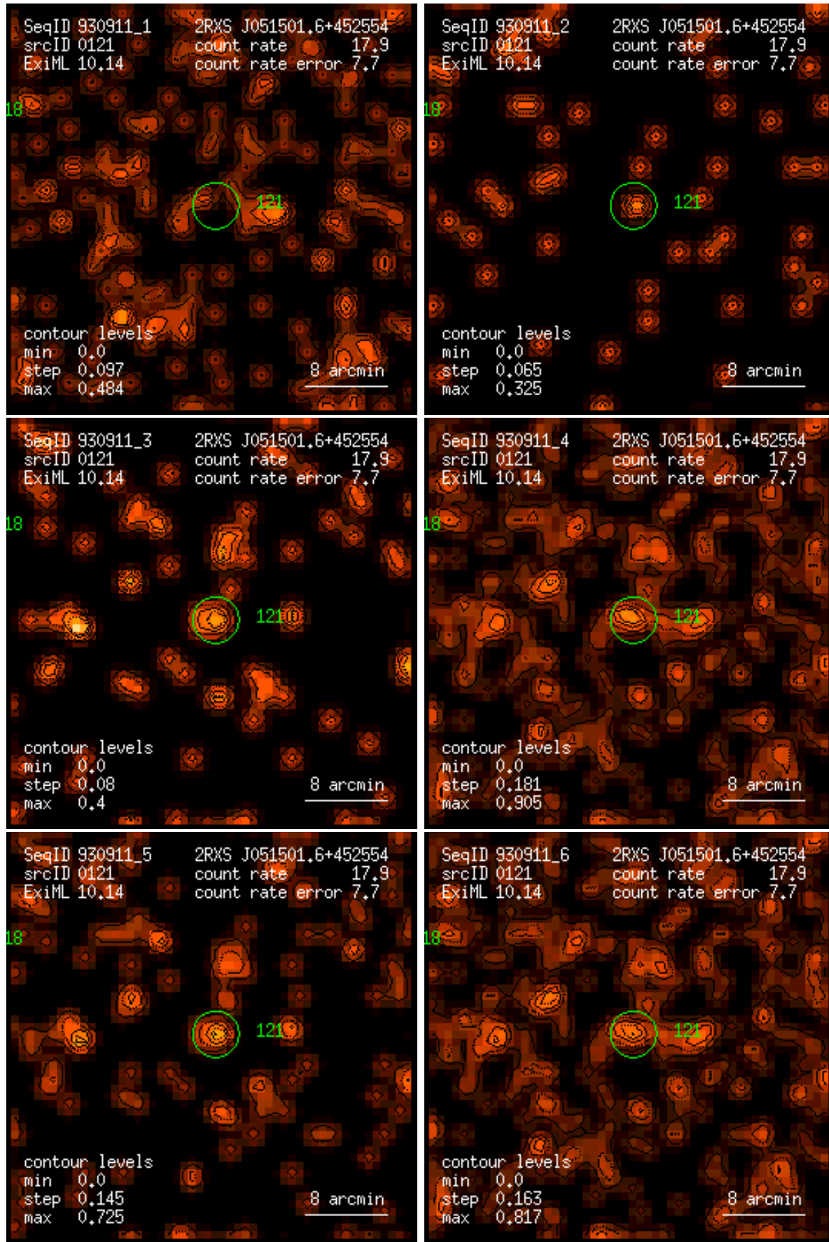
Figure 121: RASS 930911: detection 0121: band rate images, Gaussian filter: (1) PSPC channels 11 – 41, (2) 52 – 90, (3) 91 – 201, (4) 11 – 235, (5) 52 – 201, (6) 11 – 201. Broad band rates in counts/ks. Band rate contour levels in counts/ks/arcmin 2 .
