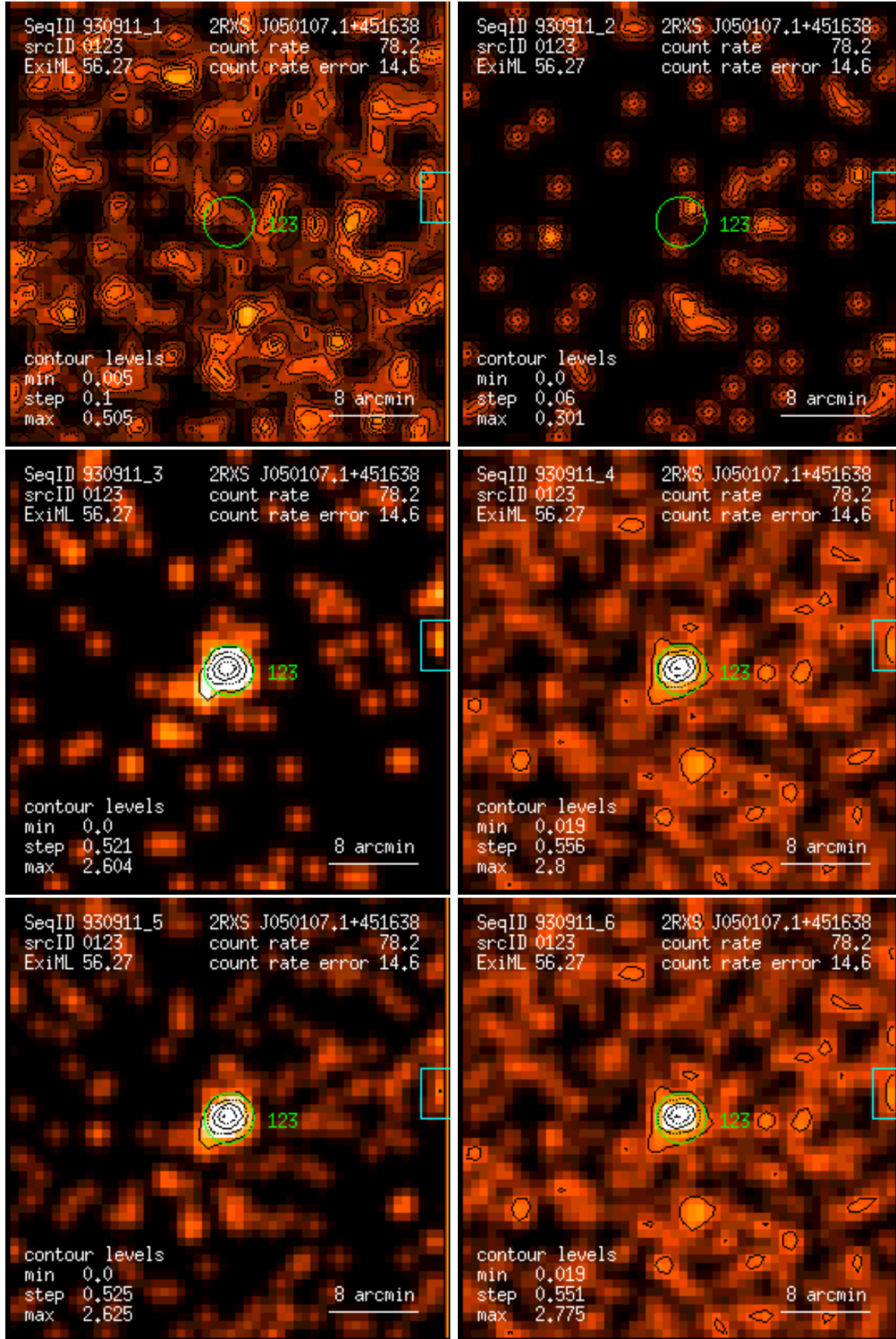
Figure 123: RASS 930911: detection 0123: band rate images, Gaussian filter: (1) PSPC channels 11 – 41, (2) 52 – 90, (3) 91 – 201, (4) 11 – 235, (5) 52 – 201, (6) 11 – 201. Broad band rates in counts/ks. Band rate contour levels in counts/ks/arcmin 2 .
