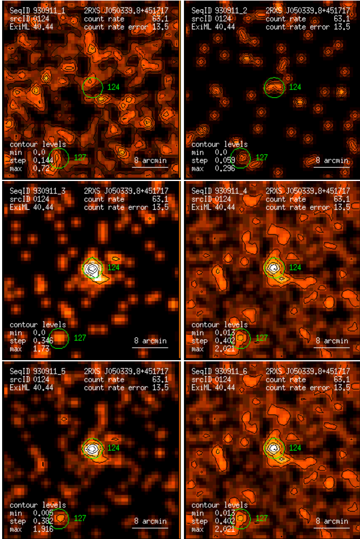
Figure 124: RASS 930911: detection 0124: band rate images, Gaussian filter: (1) PSPC channels 11 – 41, (2) 52 – 90, (3) 91 – 201, (4) 11 – 235, (5) 52 – 201, (6) 11 – 201. Broad band rates in counts/ks. Band rate contour levels in counts/ks/arcmin 2 .
