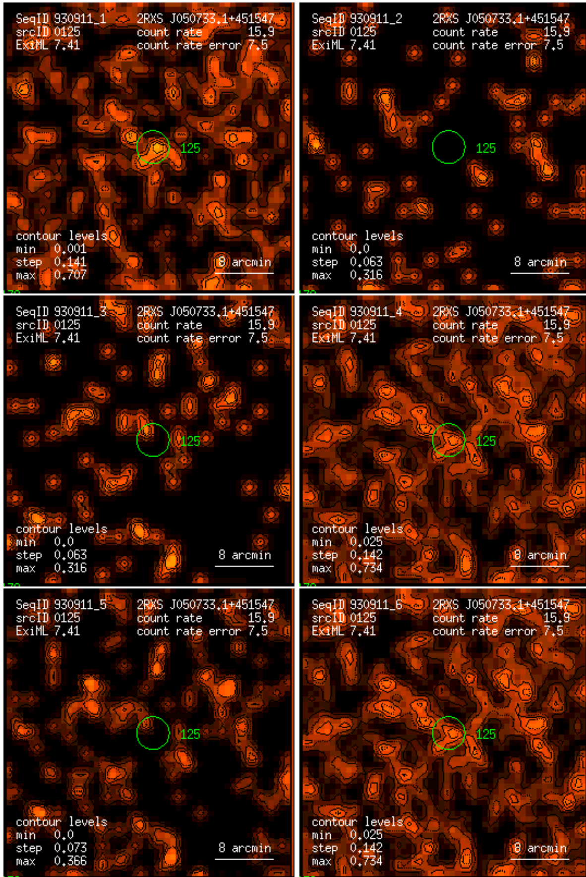
Figure 125: RASS 930911: detection 0125: band rate images, Gaussian filter: (1) PSPC channels 11 – 41, (2) 52 – 90, (3) 91 – 201, (4) 11 – 235, (5) 52 – 201, (6) 11 – 201. Broad band rates in counts/ks. Band rate contour levels in counts/ks/arcmin 2 .
