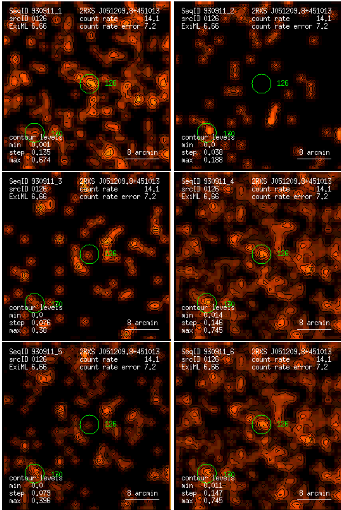
Figure 126: RASS 930911: detection 0126: band rate images, Gaussian filter: (1) PSPC channels 11 – 41, (2) 52 – 90, (3) 91 – 201, (4) 11 – 235, (5) 52 – 201, (6) 11 – 201. Broad band rates in counts/ks. Band rate contour levels in counts/ks/arcmin 2 .
