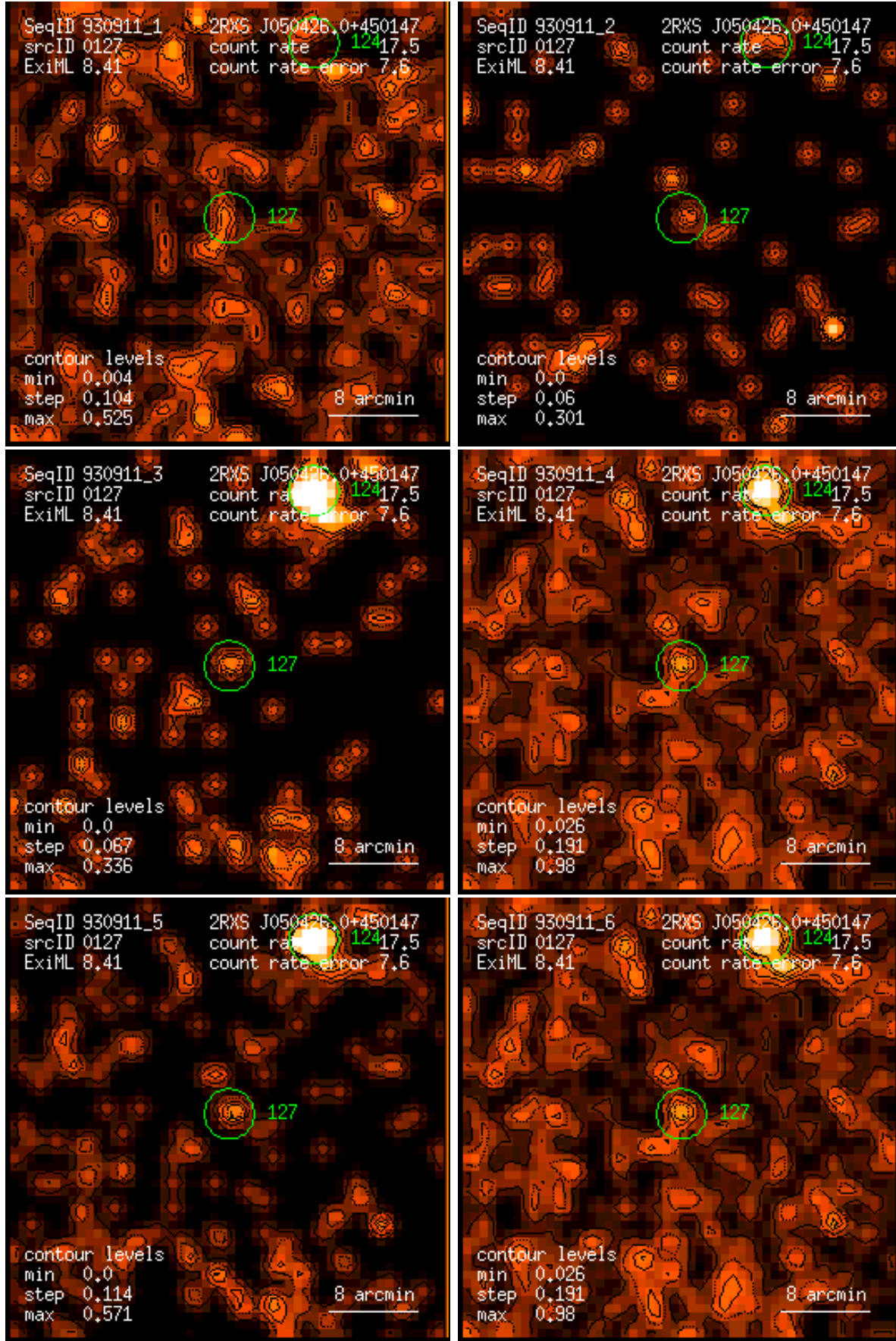
Figure 127: RASS 930911: detection 0127: band rate images, Gaussian filter: (1) PSPC channels 11 – 41, (2) 52 – 90, (3) 91 – 201, (4) 11 – 235, (5) 52 – 201, (6) 11 – 201. Broad band rates in counts/ks. Band rate contour levels in counts/ks/arcmin 2 .
