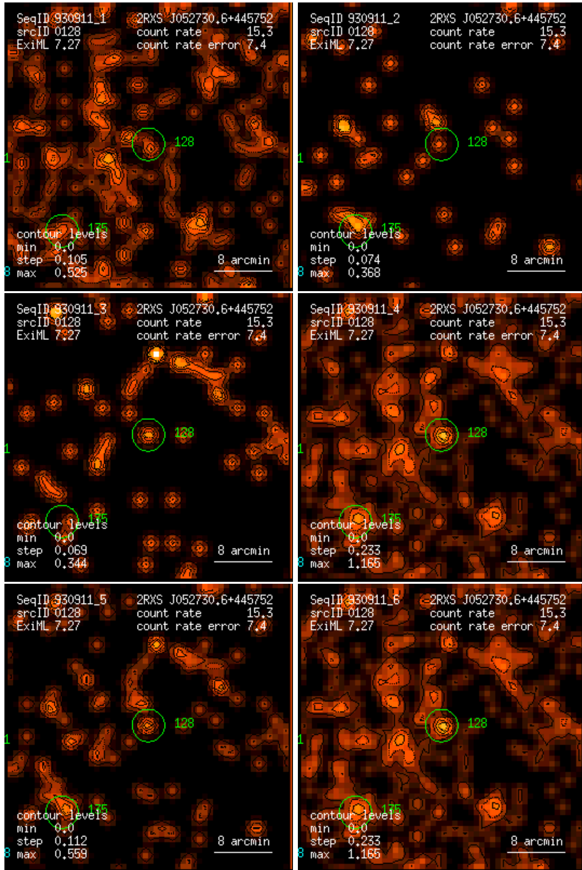
Figure 128: RASS 930911: detection 0128: band rate images, Gaussian filter: (1) PSPC channels 11 – 41, (2) 52 – 90, (3) 91 – 201, (4) 11 – 235, (5) 52 – 201, (6) 11 – 201. Broad band rates in counts/ks. Band rate contour levels in counts/ks/arcmin 2 .
