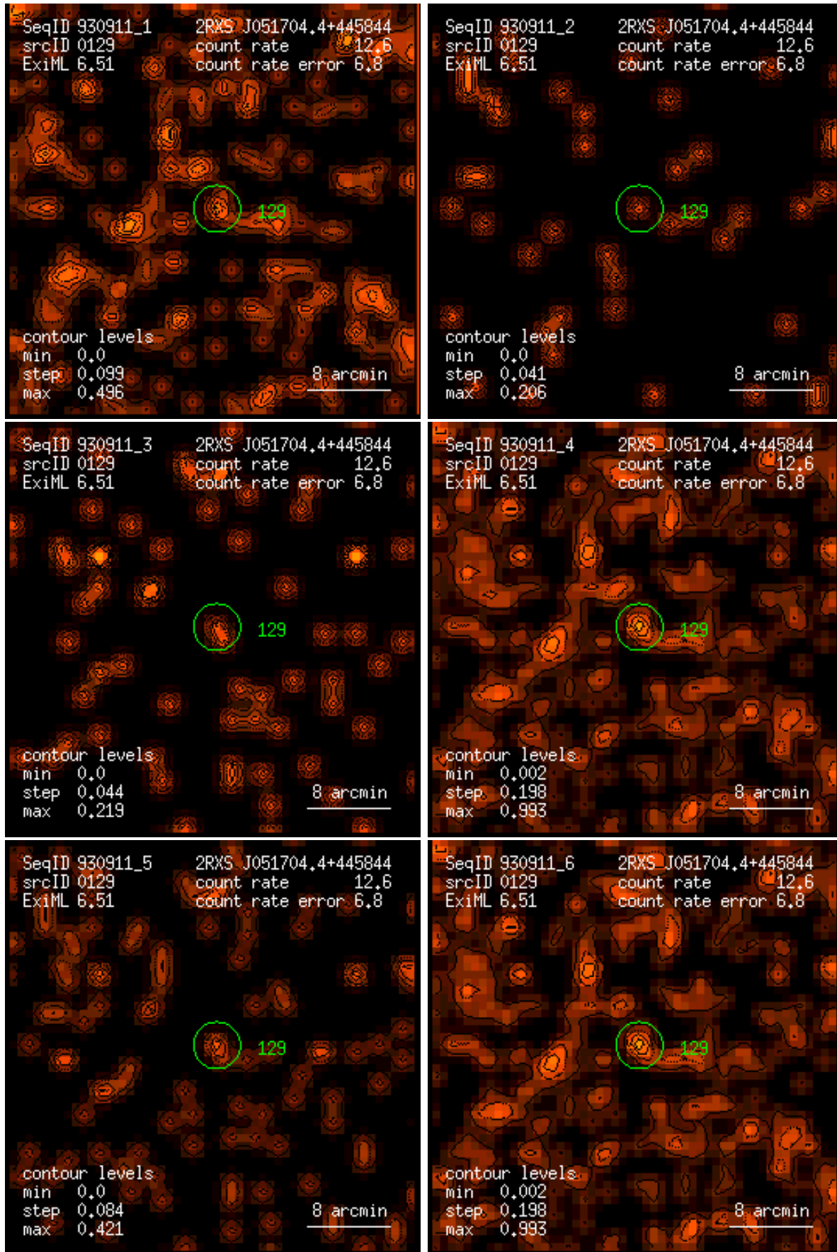
Figure 129: RASS 930911: detection 0129: band rate images, Gaussian filter: (1) PSPC channels 11 – 41, (2) 52 – 90, (3) 91 – 201, (4) 11 – 235, (5) 52 – 201, (6) 11 – 201. Broad band rates in counts/ks. Band rate contour levels in counts/ks/arcmin 2 .
