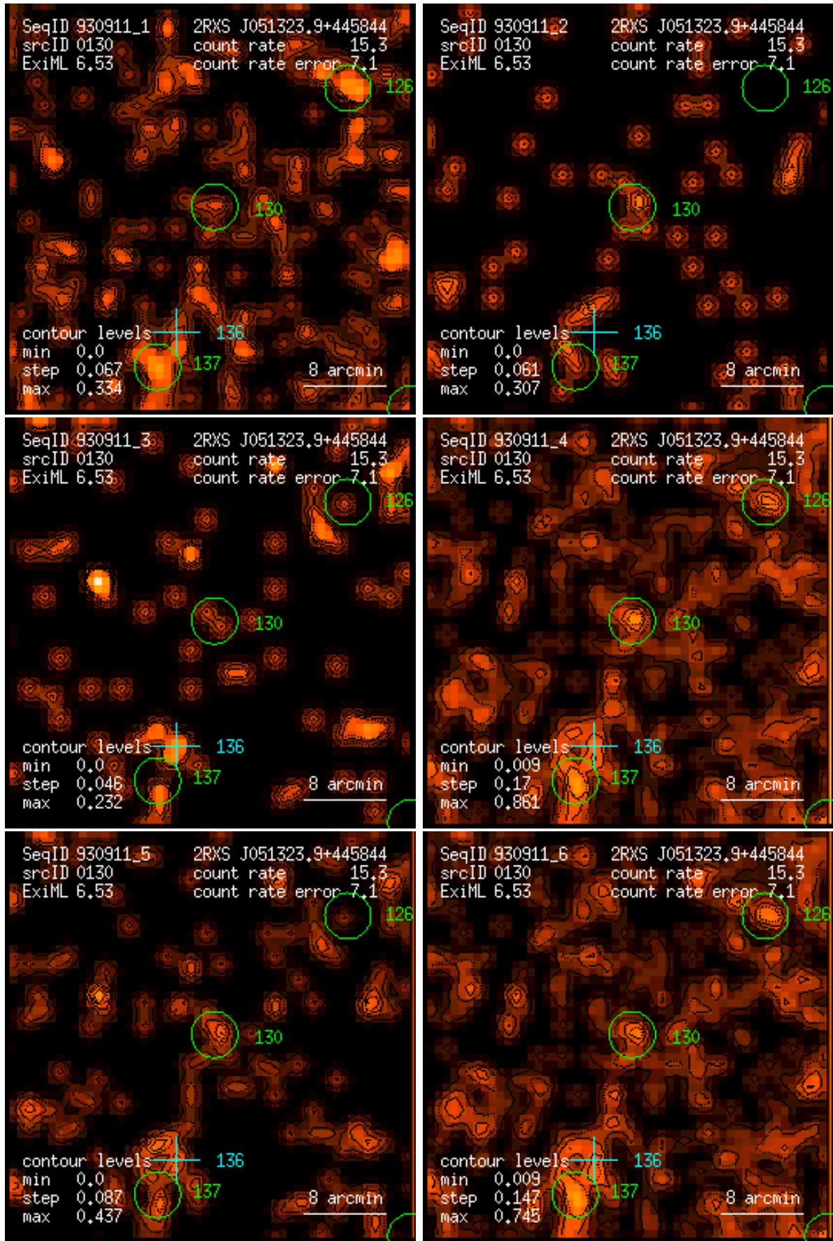
Figure 130: RASS 930911: detection 0130: band rate images, Gaussian filter: (1) PSPC channels 11 – 41, (2) 52 – 90, (3) 91 – 201, (4) 11 – 235, (5) 52 – 201, (6) 11 – 201. Broad band rates in counts/ks. Band rate contour levels in counts/ks/arcmin 2 .
