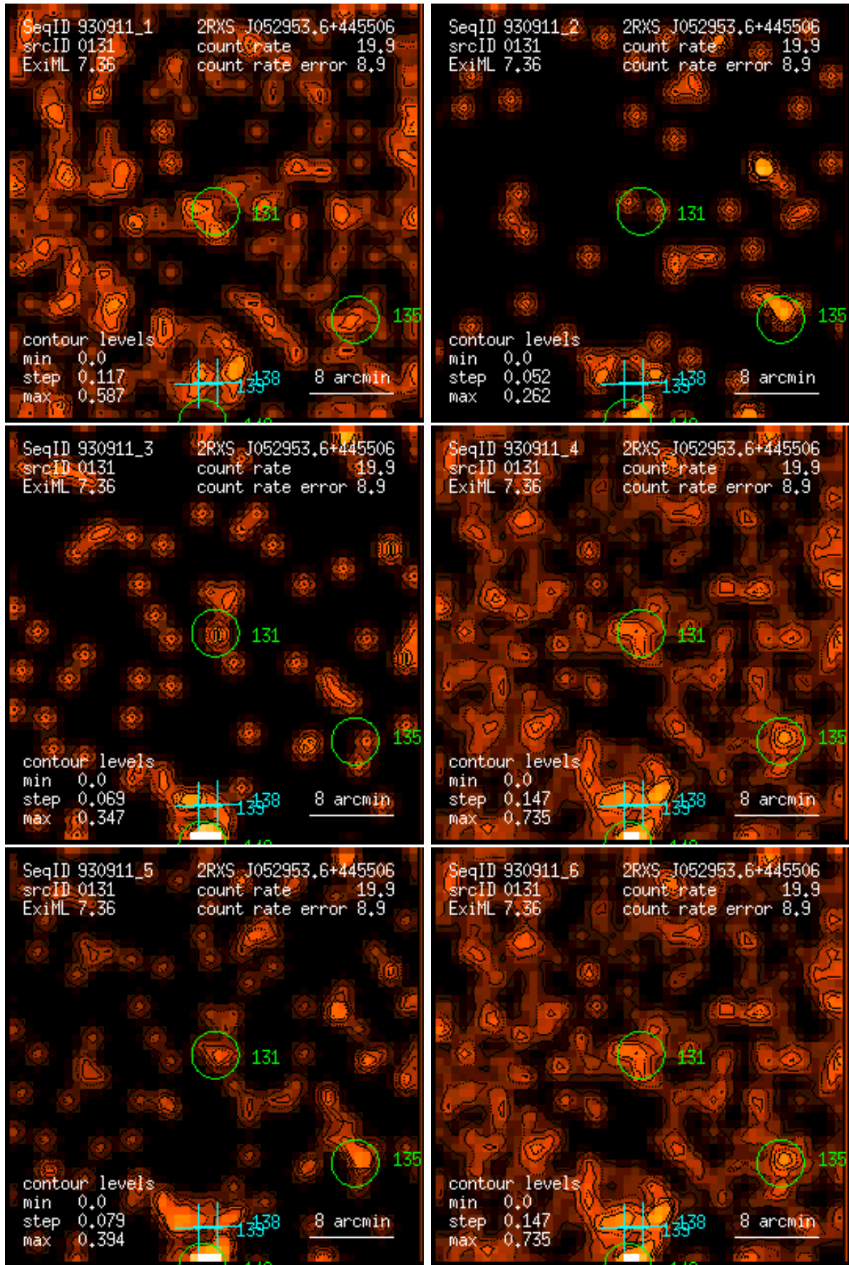
Figure 131: RASS 930911: detection 0131: band rate images, Gaussian filter: (1) PSPC channels 11 – 41, (2) 52 – 90, (3) 91 – 201, (4) 11 – 235, (5) 52 – 201, (6) 11 – 201. Broad band rates in counts/ks. Band rate contour levels in counts/ks/arcmin 2 .
