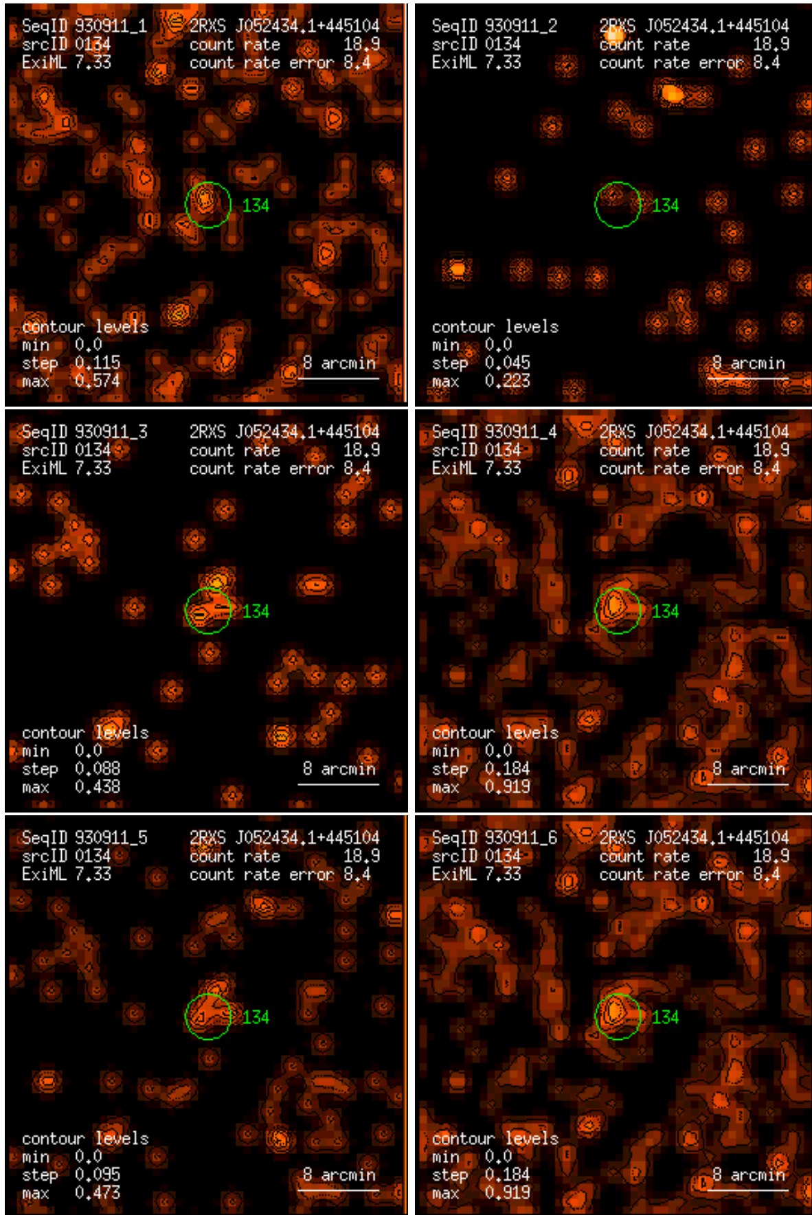
Figure 134: RASS 930911: detection 0134: band rate images, Gaussian filter: (1) PSPC channels 11 – 41, (2) 52 – 90, (3) 91 – 201, (4) 11 – 235, (5) 52 – 201, (6) 11 – 201. Broad band rates in counts/ks. Band rate contour levels in counts/ks/arcmin 2 .
