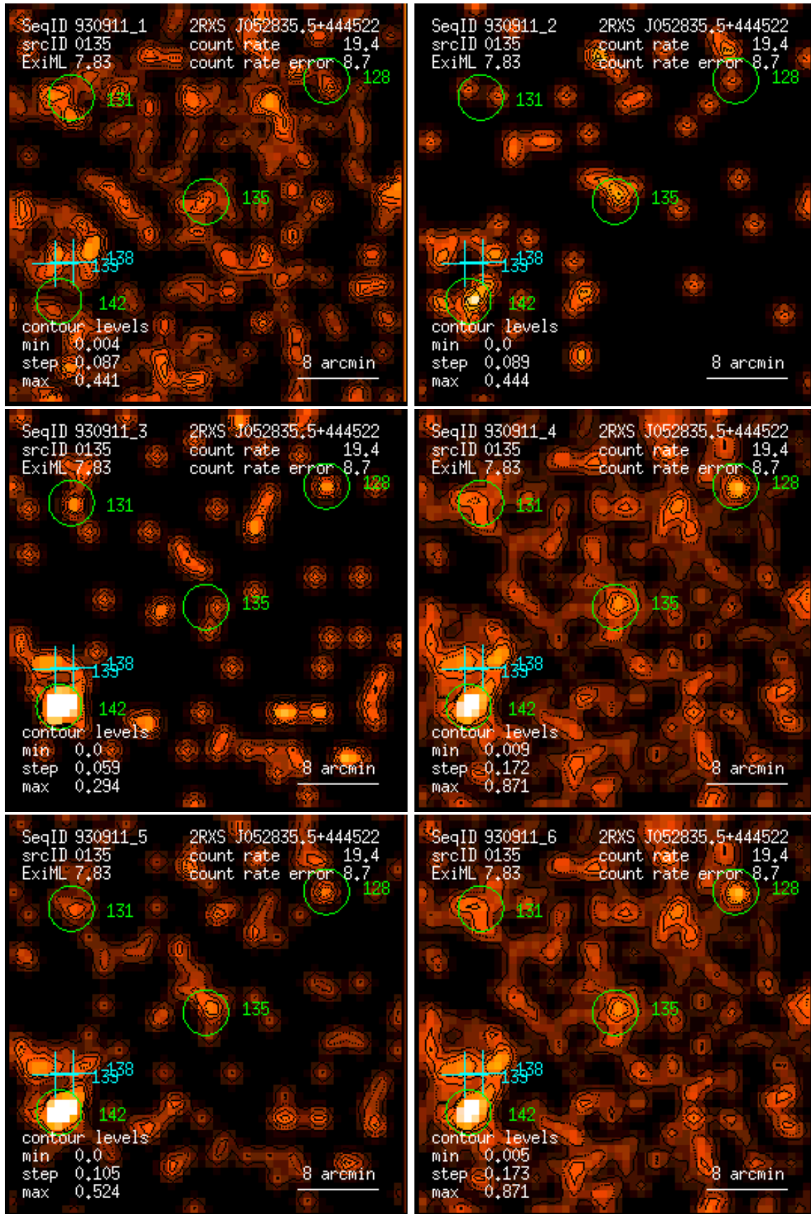
Figure 135: RASS 930911: detection 0135: band rate images, Gaussian filter: (1) PSPC channels 11 – 41, (2) 52 – 90, (3) 91 – 201, (4) 11 – 235, (5) 52 – 201, (6) 11 – 201. Broad band rates in counts/ks. Band rate contour levels in counts/ks/arcmin 2 .
