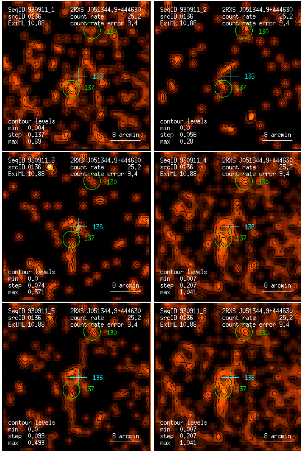
Figure 136: RASS 930911: detection 0136: band rate images, Gaussian filter: (1) PSPC channels 11 – 41, (2) 52 – 90, (3) 91 – 201, (4) 11 – 235, (5) 52 – 201, (6) 11 – 201. Broad band rates in counts/ks. Band rate contour levels in counts/ks/arcmin 2 .
