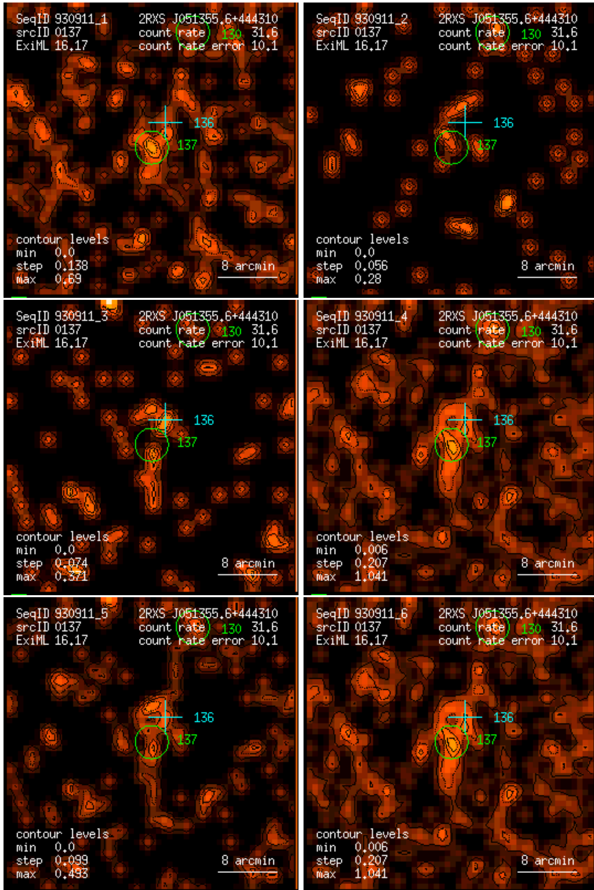
Figure 137: RASS 930911: detection 0137: band rate images, Gaussian filter: (1) PSPC channels 11 – 41, (2) 52 – 90, (3) 91 – 201, (4) 11 – 235, (5) 52 – 201, (6) 11 – 201. Broad band rates in counts/ks. Band rate contour levels in counts/ks/arcmin 2 .
