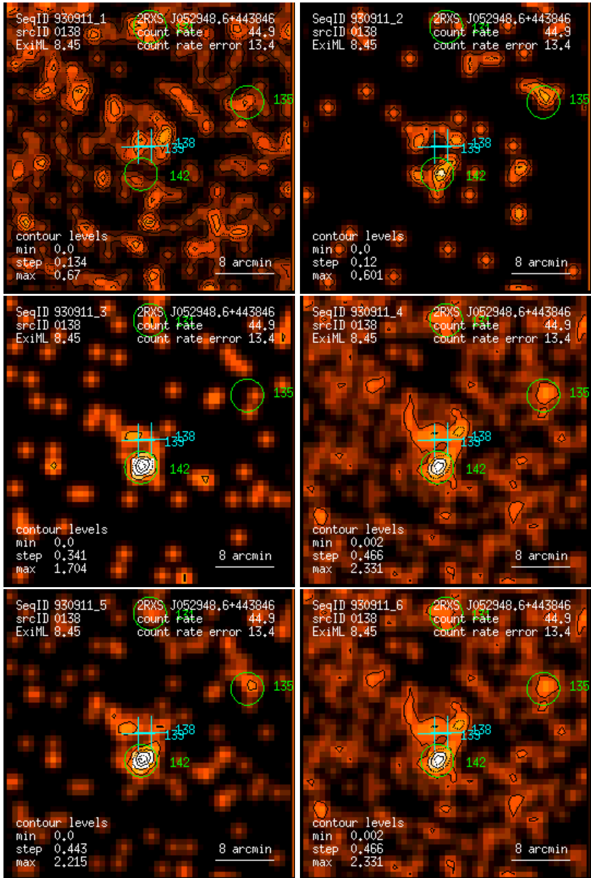
Figure 138: RASS 930911: detection 0138: band rate images, Gaussian filter: (1) PSPC channels 11 – 41, (2) 52 – 90, (3) 91 – 201, (4) 11 – 235, (5) 52 – 201, (6) 11 – 201. Broad band rates in counts/ks. Band rate contour levels in counts/ks/arcmin 2 .
