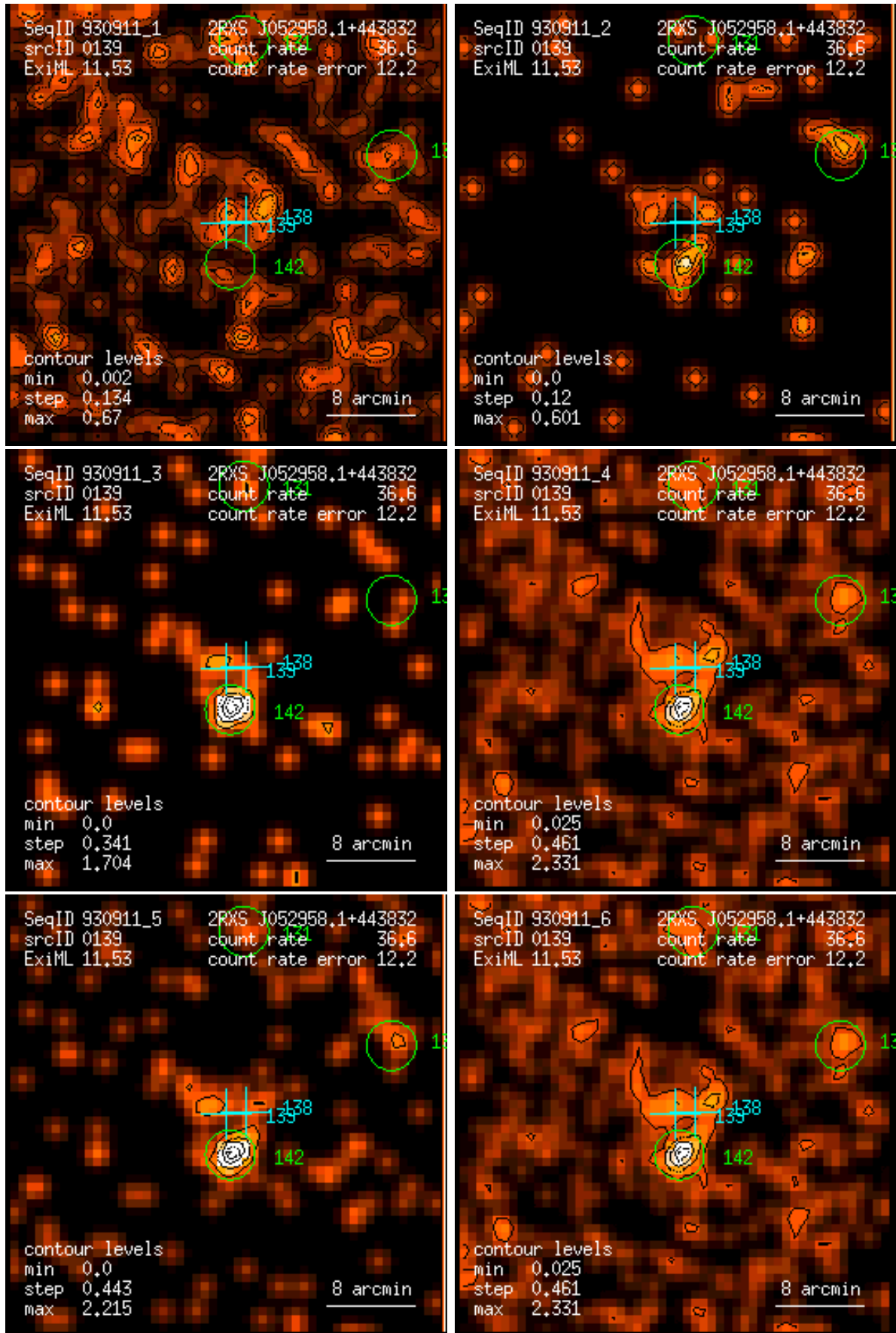
Figure 139: RASS 930911: detection 0139: band rate images, Gaussian filter: (1) PSPC channels 11 – 41, (2) 52 – 90, (3) 91 – 201, (4) 11 – 235, (5) 52 – 201, (6) 11 – 201. Broad band rates in counts/ks. Band rate contour levels in counts/ks/arcmin 2 .
