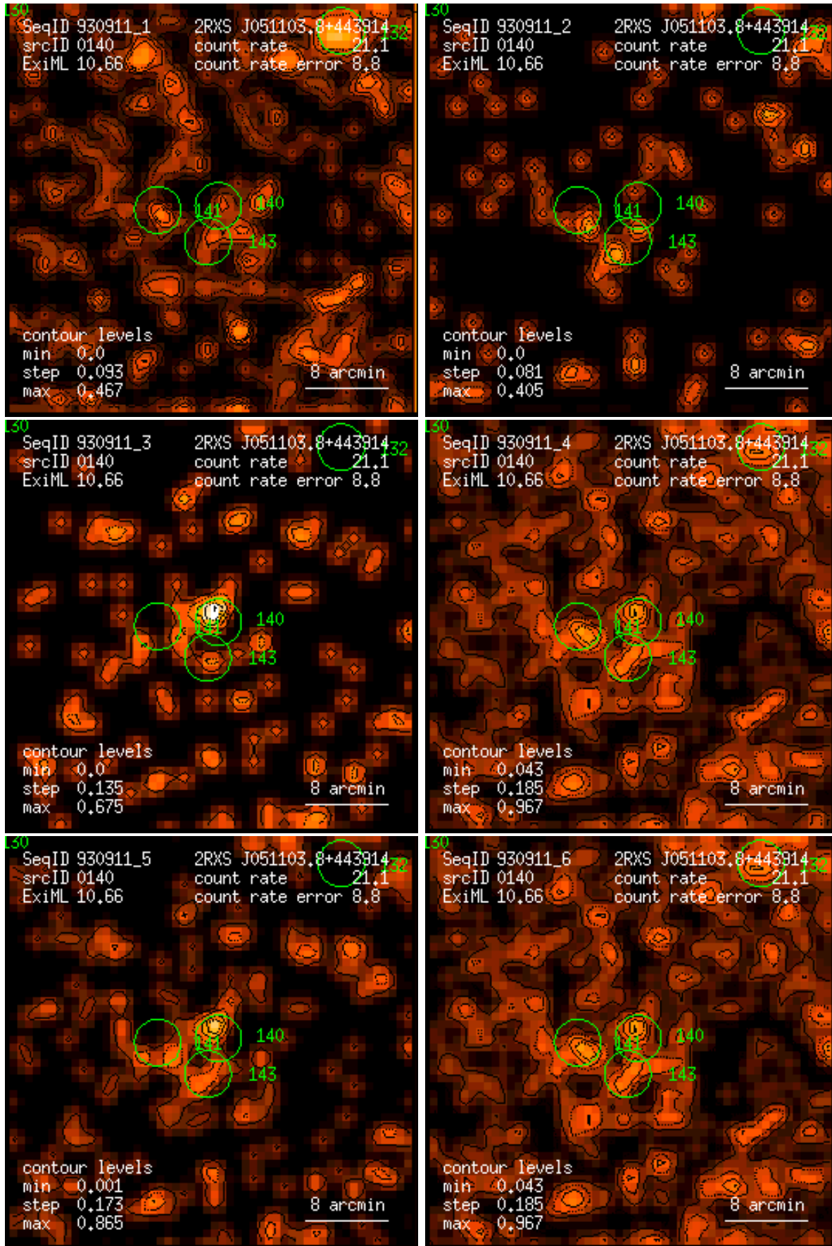
Figure 140: RASS 930911: detection 0140: band rate images, Gaussian filter: (1) PSPC channels 11 – 41, (2) 52 – 90, (3) 91 – 201, (4) 11 – 235, (5) 52 – 201, (6) 11 – 201. Broad band rates in counts/ks. Band rate contour levels in counts/ks/arcmin 2 .
