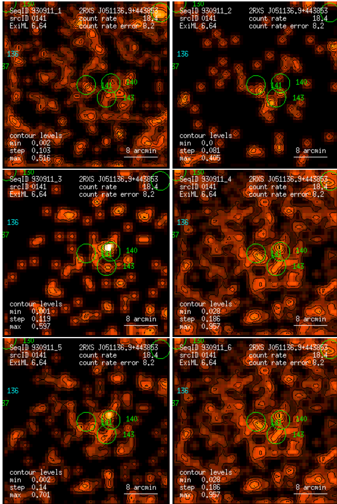
Figure 141: RASS 930911: detection 0141: band rate images, Gaussian filter: (1) PSPC channels 11 – 41, (2) 52 – 90, (3) 91 – 201, (4) 11 – 235, (5) 52 – 201, (6) 11 – 201. Broad band rates in counts/ks. Band rate contour levels in counts/ks/arcmin 2 .
