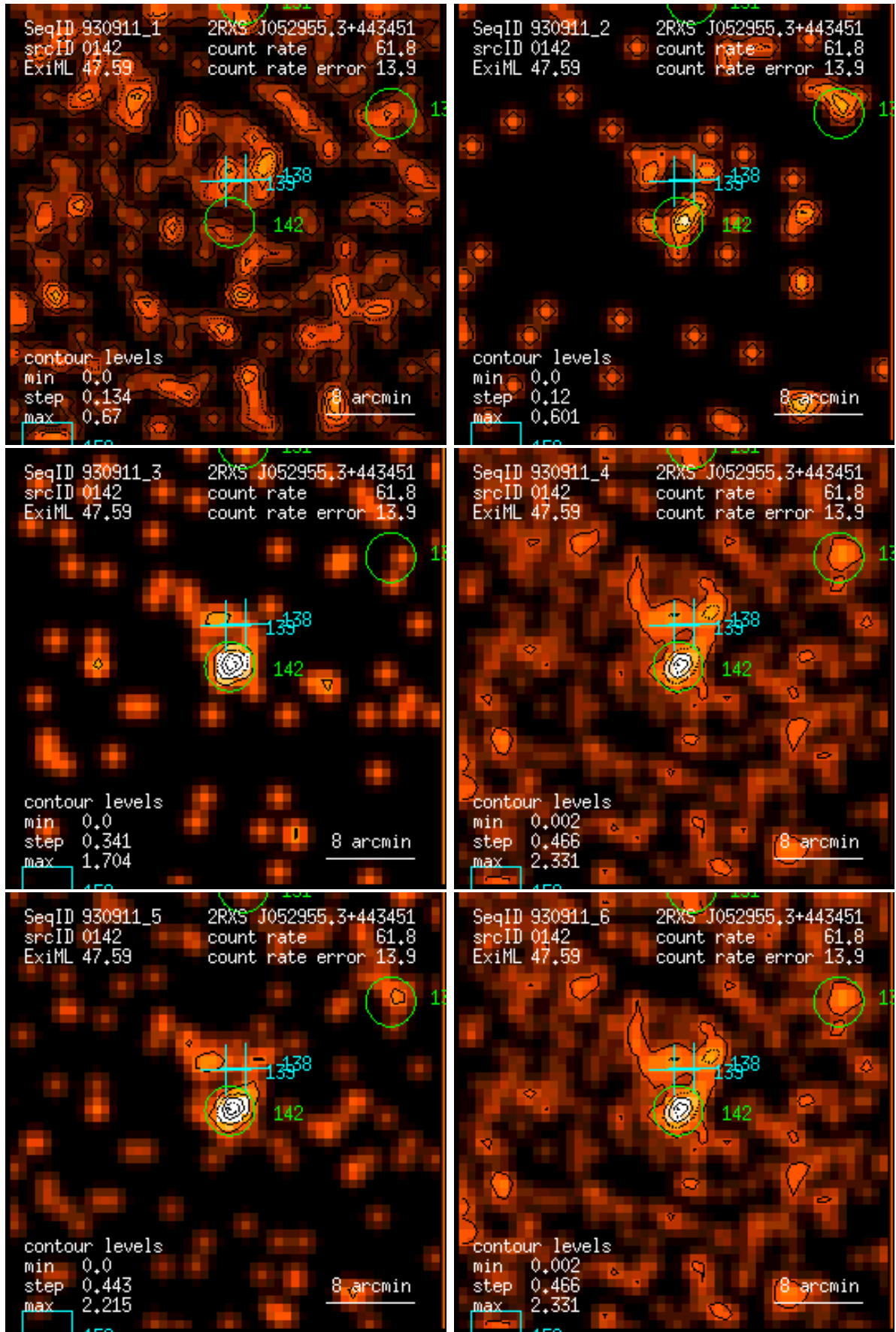
Figure 142: RASS 930911: detection 0142: band rate images, Gaussian filter: (1) PSPC channels 11 – 41, (2) 52 – 90, (3) 91 – 201, (4) 11 – 235, (5) 52 – 201, (6) 11 – 201. Broad band rates in counts/ks. Band rate contour levels in counts/ks/arcmin 2 .
