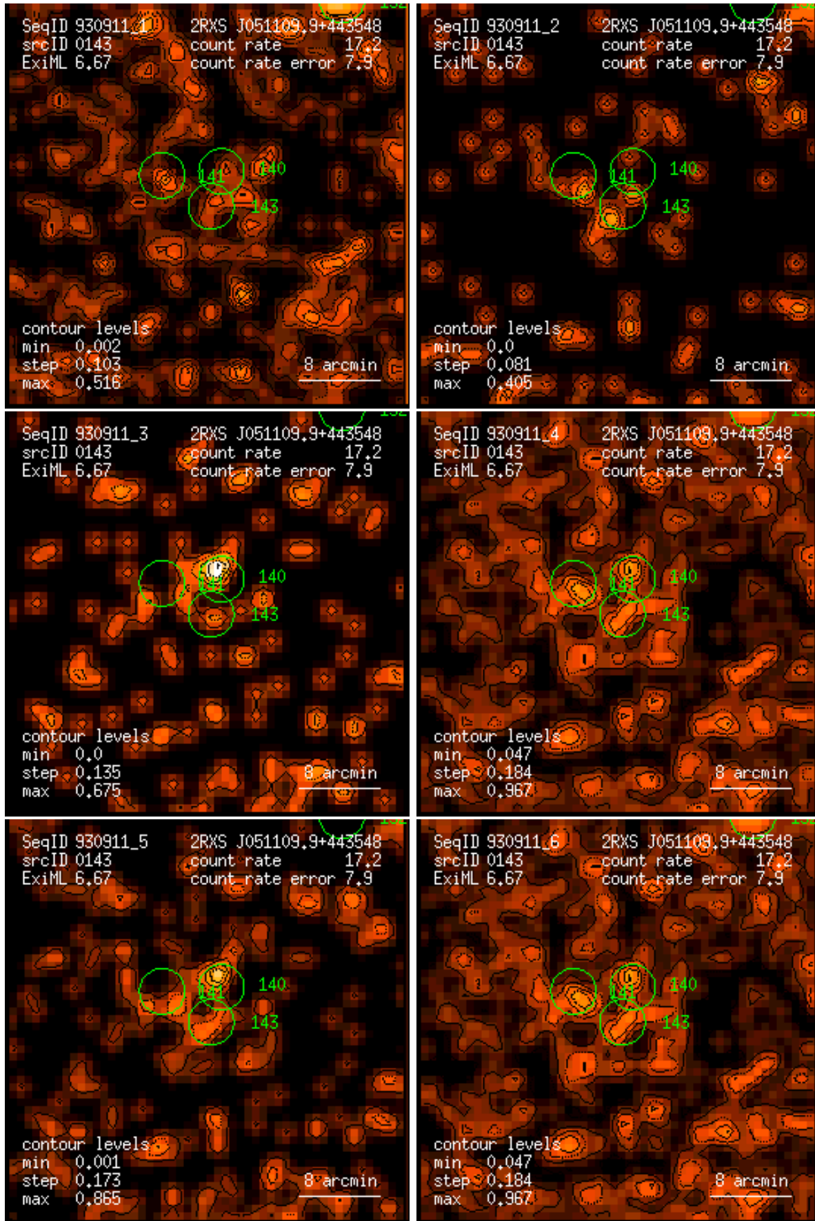
Figure 143: RASS 930911: detection 0143: band rate images, Gaussian filter: (1) PSPC channels 11 – 41, (2) 52 – 90, (3) 91 – 201, (4) 11 – 235, (5) 52 – 201, (6) 11 – 201. Broad band rates in counts/ks. Band rate contour levels in counts/ks/arcmin 2 .
