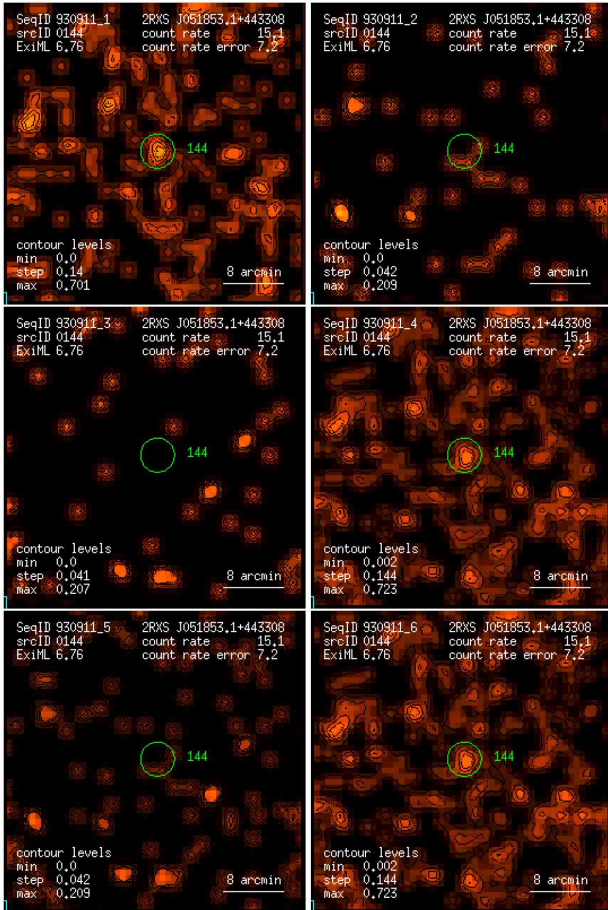
Figure 144: RASS 930911: detection 0144: band rate images, Gaussian filter: (1) PSPC channels 11 – 41, (2) 52 – 90, (3) 91 – 201, (4) 11 – 235, (5) 52 – 201, (6) 11 – 201. Broad band rates in counts/ks. Band rate contour levels in counts/ks/arcmin 2 .
