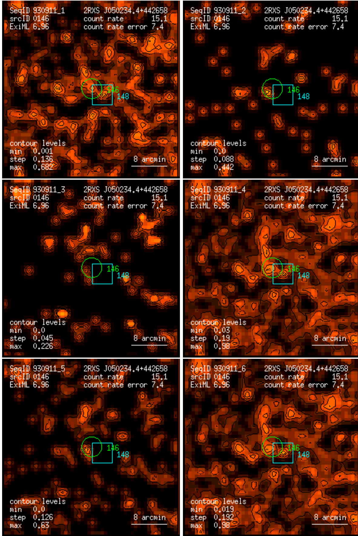
Figure 146: RASS 930911: detection 0146: band rate images, Gaussian filter: (1) PSPC channels 11 – 41, (2) 52 – 90, (3) 91 – 201, (4) 11 – 235, (5) 52 – 201, (6) 11 – 201. Broad band rates in counts/ks. Band rate contour levels in counts/ks/arcmin 2 .
