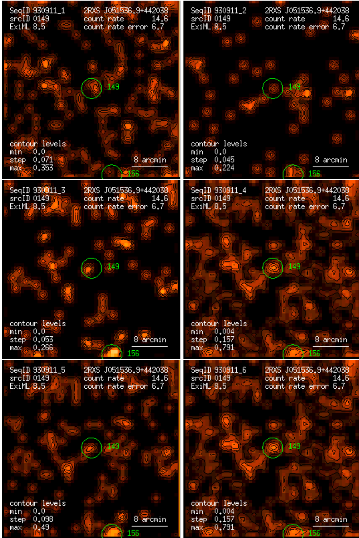
Figure 149: RASS 930911: detection 0149: band rate images, Gaussian filter: (1) PSPC channels 11 – 41, (2) 52 – 90, (3) 91 – 201, (4) 11 – 235, (5) 52 – 201, (6) 11 – 201. Broad band rates in counts/ks. Band rate contour levels in counts/ks/arcmin 2 .
