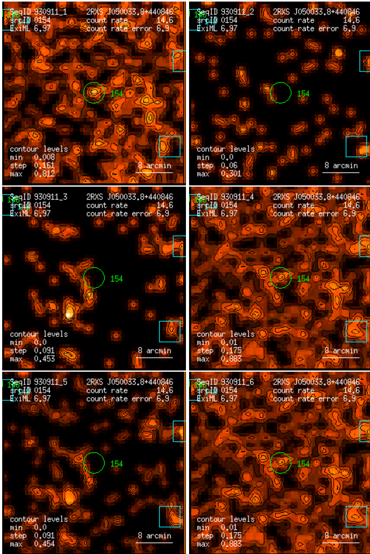
Figure 154: RASS 930911: detection 0154: band rate images, Gaussian filter: (1) PSPC channels 11 – 41, (2) 52 – 90, (3) 91 – 201, (4) 11 – 235, (5) 52 – 201, (6) 11 – 201. Broad band rates in counts/ks. Band rate contour levels in counts/ks/arcmin 2 .
