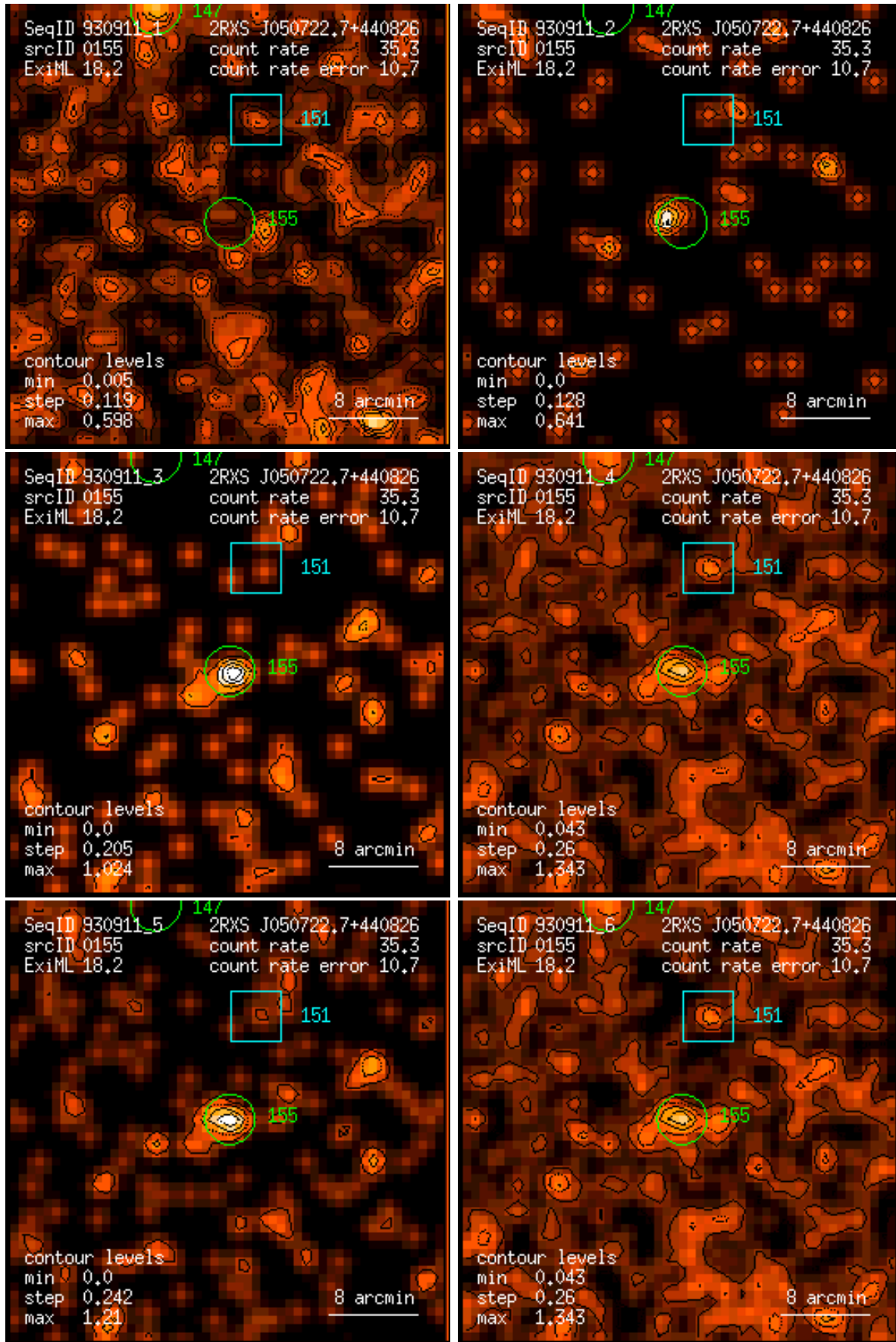
Figure 155: RASS 930911: detection 0155: band rate images, Gaussian filter: (1) PSPC channels 11 – 41, (2) 52 – 90, (3) 91 – 201, (4) 11 – 235, (5) 52 – 201, (6) 11 – 201. Broad band rates in counts/ks. Band rate contour levels in counts/ks/arcmin 2 .
