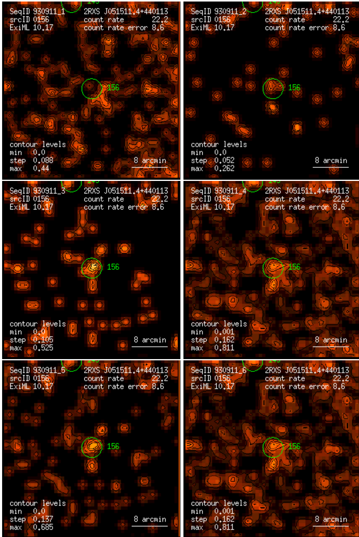
Figure 156: RASS 930911: detection 0156: band rate images, Gaussian filter: (1) PSPC channels 11 – 41, (2) 52 – 90, (3) 91 – 201, (4) 11 – 235, (5) 52 – 201, (6) 11 – 201. Broad band rates in counts/ks. Band rate contour levels in counts/ks/arcmin 2 .
