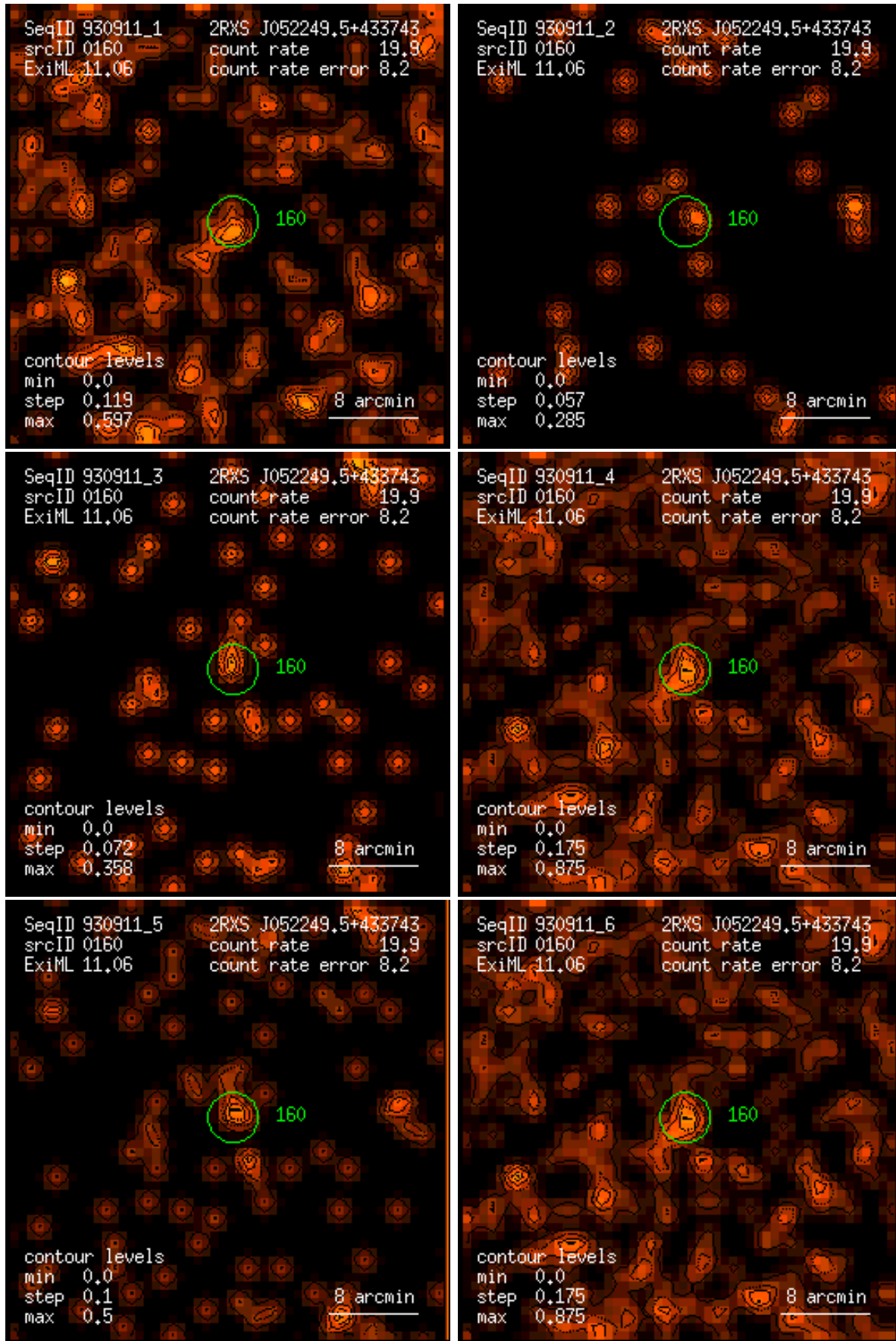
Figure 160: RASS 930911: detection 0160: band rate images, Gaussian filter: (1) PSPC channels 11 – 41, (2) 52 – 90, (3) 91 – 201, (4) 11 – 235, (5) 52 – 201, (6) 11 – 201. Broad band rates in counts/ks. Band rate contour levels in counts/ks/arcmin 2 .
