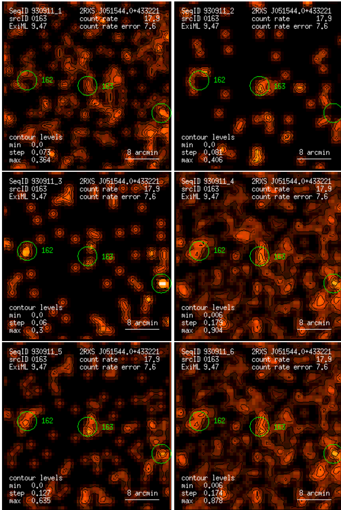
Figure 163: RASS 930911: detection 0163: band rate images, Gaussian filter: (1) PSPC channels 11 – 41, (2) 52 – 90, (3) 91 – 201, (4) 11 – 235, (5) 52 – 201, (6) 11 – 201. Broad band rates in counts/ks. Band rate contour levels in counts/ks/arcmin 2 .
