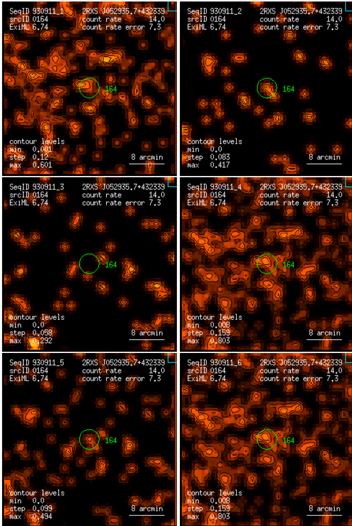
Figure 164: RASS 930911: detection 0164: band rate images, Gaussian filter: (1) PSPC channels 11 – 41, (2) 52 – 90, (3) 91 – 201, (4) 11 – 235, (5) 52 – 201, (6) 11 – 201. Broad band rates in counts/ks. Band rate contour levels in counts/ks/arcmin 2 .
