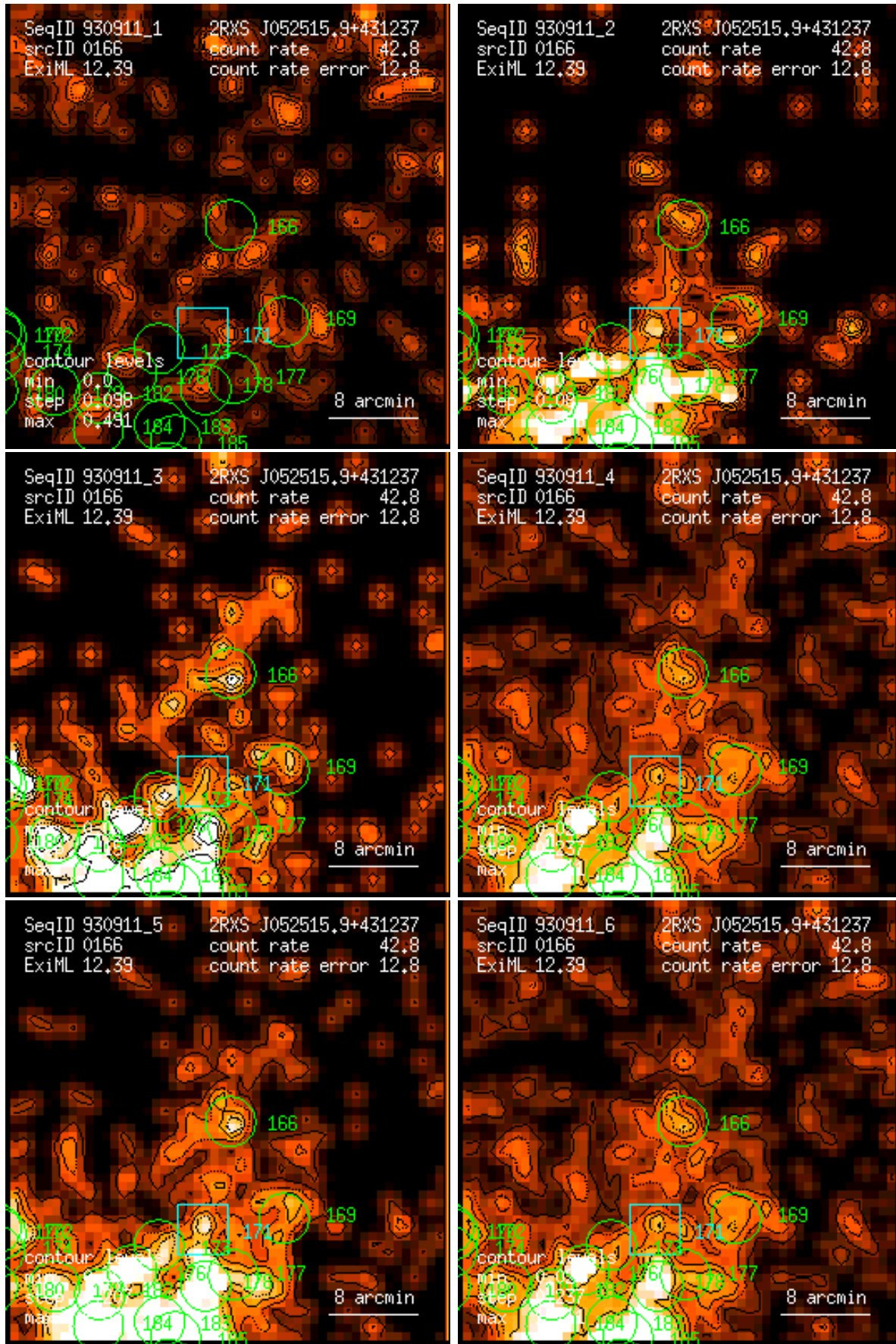
Figure 166: RASS 930911: detection 0166: band rate images, Gaussian filter: (1) PSPC channels 11 – 41, (2) 52 – 90, (3) 91 – 201, (4) 11 – 235, (5) 52 – 201, (6) 11 – 201. Broad band rates in counts/ks. Band rate contour levels in counts/ks/arcmin 2 .
